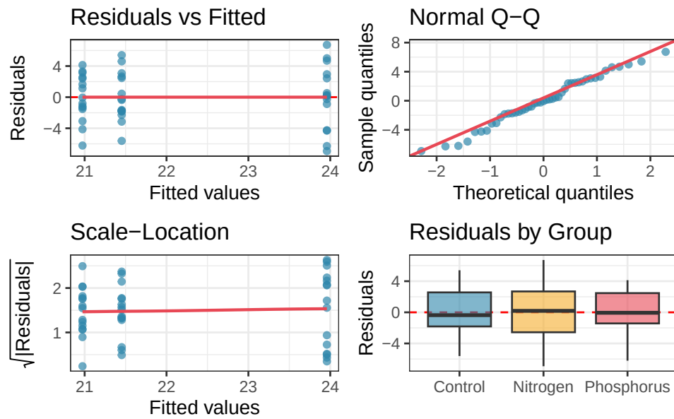
Figure 2.10: Four residual diagnostic plots for a one-way ANOVA fitted to the fertiliser data. Top left: residuals vs fitted values — roughly equal spread across groups confirms homoscedasticity. Top right: Q-Q plot, points close to the line confirm approximate normality. Bottom left: scale-location plot, a flat trend confirms homoscedasticity. Bottom right: residuals by group, box heights are similar and no extreme outliers are present.
