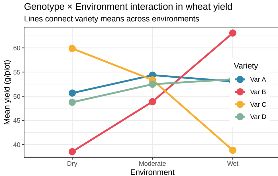
Figure 5.4: Genotype by environment interaction plot for four wheat varieties across three rainfall environments. Lines connect the mean yield of each variety across environments. Var B and Var C show a clear crossover interaction: Var C outperforms Var B in dry conditions while Var B outperforms Var C in wet conditions. Var A and Var D are stable across environments. A breeder seeking a universally adapted variety would recommend Var A or Var D; recommendations for Var B or Var C must be environment-specific.
