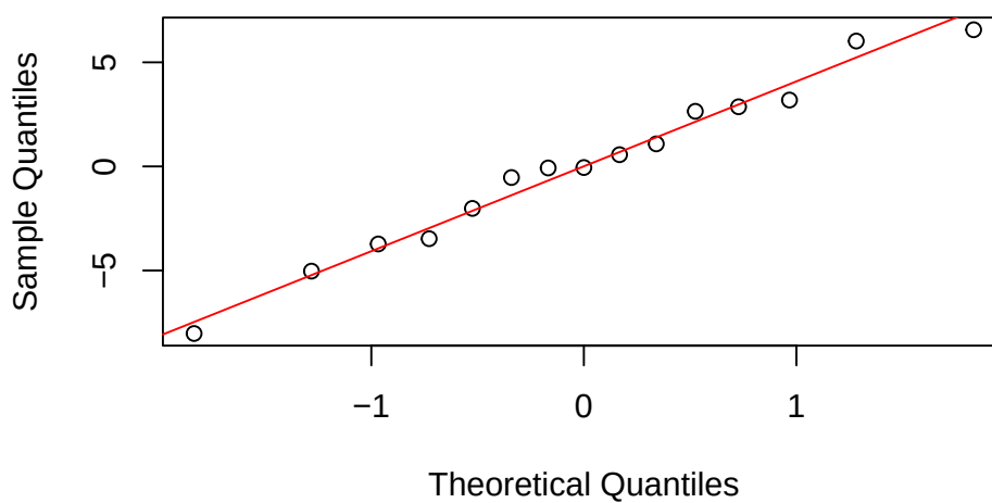
Q-Q plot: hospital random effects
