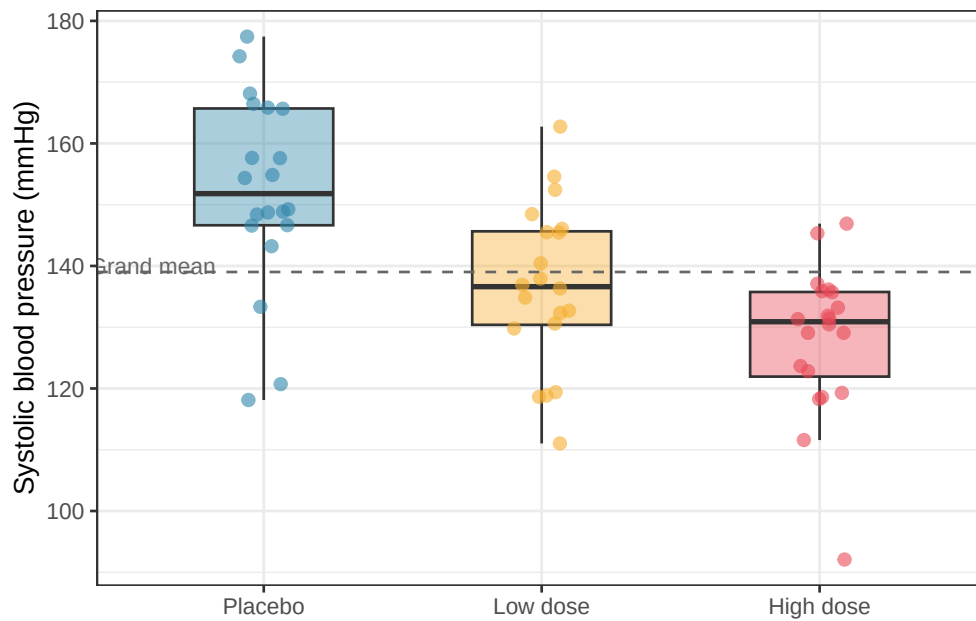
Figure 3.1.: Systolic blood pressure (mmHg) by treatment group. Individual observations are shown as points, jittered horizontally to reduce overplotting. The horizontal dashed line marks the grand mean. Even before any formal test, the progressive decrease in both the median and spread of values from placebo to high dose is clearly visible.
