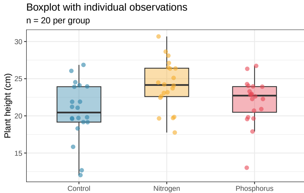
Figure 13.2.: Boxplot with individual observations overlaid for the fertiliser experiment. The boxplot shows the median, interquartile range, and outliers; the jittered points show every individual observation. This combination is the minimum acceptable display for biological data.
