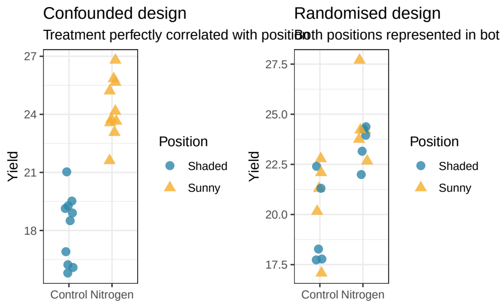
Figure 12.2.: Confounding illustrated. Left: a confounded design where all Control plants are on the shaded side of the greenhouse and all Nitrogen plants are on the sunny side. Any observed difference conflates treatment with light availability. Right: a properly randomised design where both treatments are represented on both sides, eliminating the confound.
