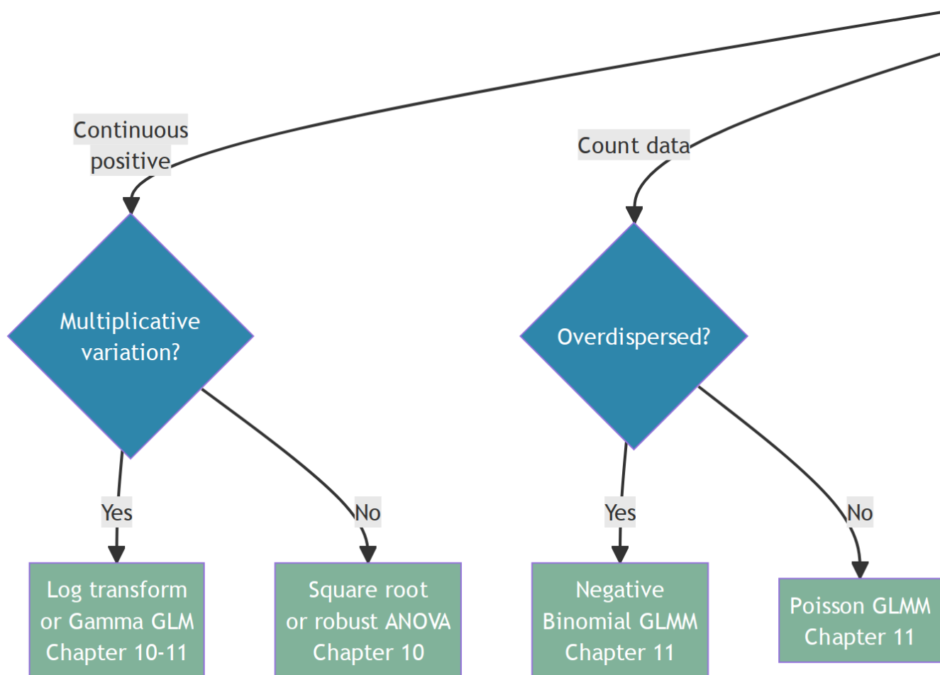
Figure C.3.: Decision tree for choosing an analysis strategy when ANOVA assumptions are violated. The choice depends primarily on the type of response variable and the nature of the violation.
