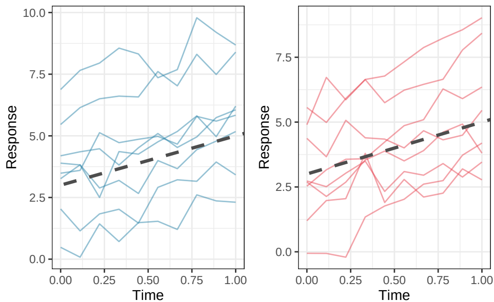
Figure 9.1.: Left: a random intercept model, all groups share the same slope but have different intercepts. The dashed line is the population-level (fixed effect) trajectory; solid lines are group-specific trajectories. Right: a random slope model, groups differ in both their starting level and their rate of change. The variation in slopes is itself a scientifically meaningful quantity.
