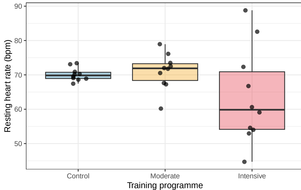
Figure 2.2.: Simulated heart rate data from one realisation of the three-group experiment. The groups share the same true mean but differ dramatically in their spread. This pattern, wider scatter in one group than another, is the signature of heteroscedasticity.
