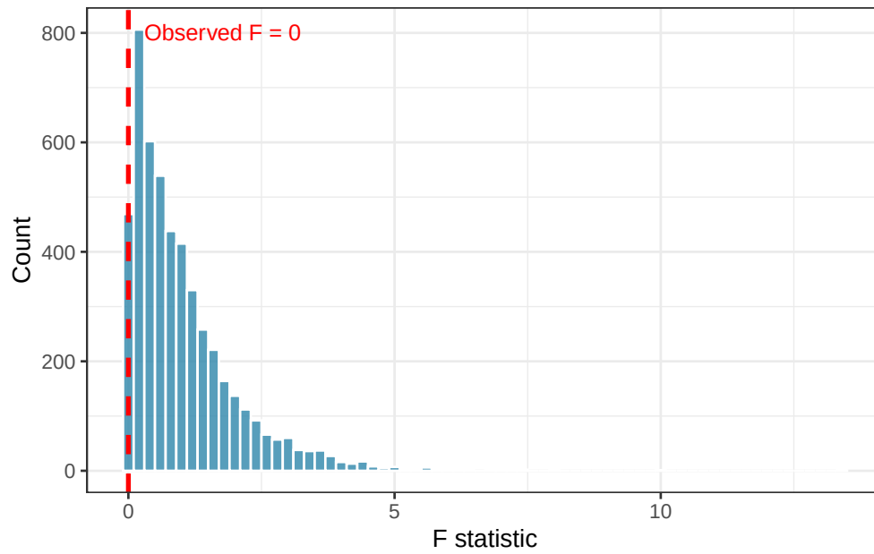
Figure 10.2.: Permutation distribution of the F statistic under the null hypothesis (4999 permutations). The red dashed line marks the observed F statistic. The permutation p-value is the proportion of permuted F values to the right of this line.
