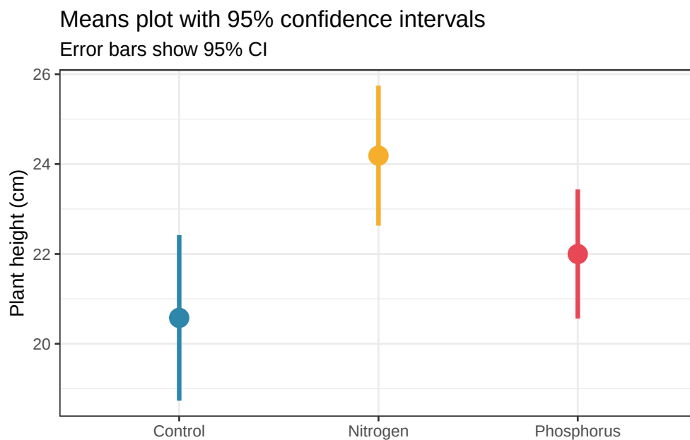
Figure 13.1.: Means plot with 95% confidence intervals for the fertiliser experiment. While compact and familiar, this format hides the distribution of the data, two datasets with identical means and CIs can have completely different distributions. Use with caution and always accompany with a more informative display.
