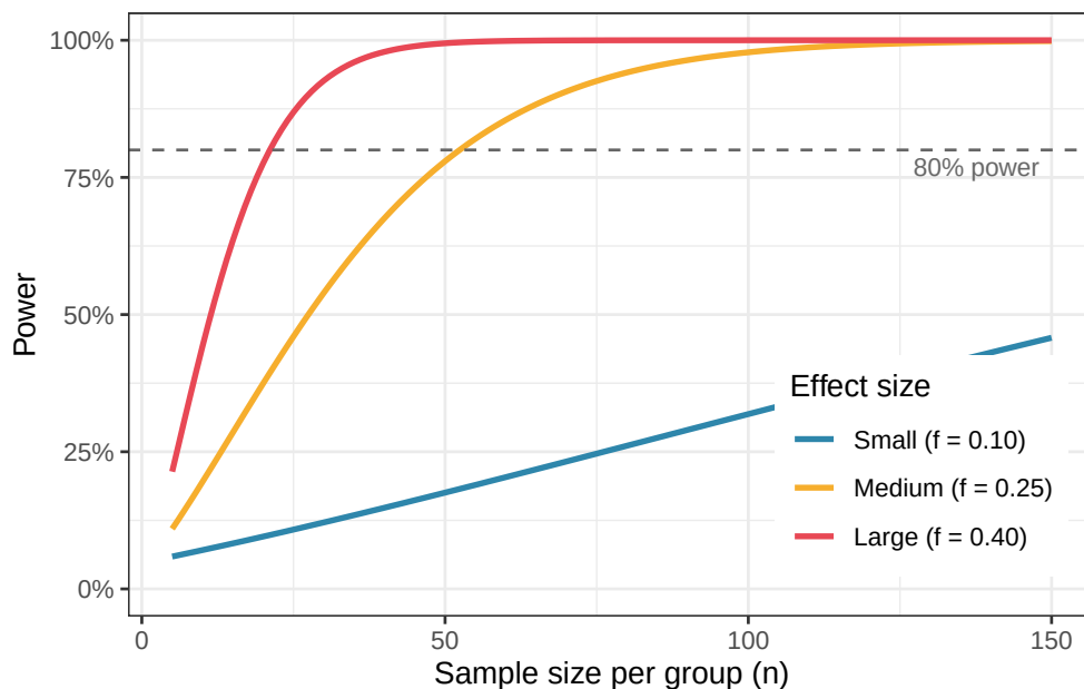
Figure 3.3.: Power curves for a one-way ANOVA with three groups at \alpha = 0.05 , across a range of sample sizes per group and for three effect sizes. The horizontal dashed line marks the conventional 80% power threshold. A medium effect requires around 52 observations per group to achieve 80% power; a small effect requires over 300.
