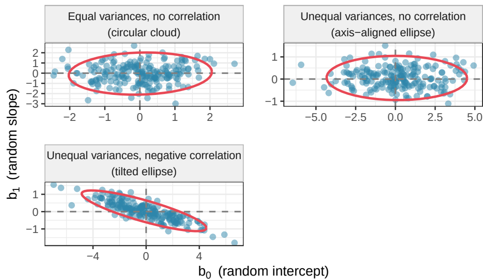
Random effect distributions under different G matrices
