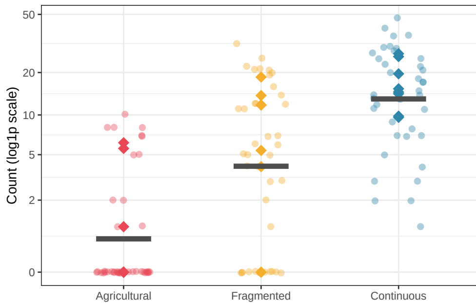
Figure 11.2.: Bird abundance counts by landscape type. The high proportion of zeros in agricultural sites (many transects showing no detections) relative to continuous forest sites illustrates the zero-inflation structure: many agricultural sites are genuinely unoccupied by this forest interior specialist. Diamonds = site means; bars = landscape means.
