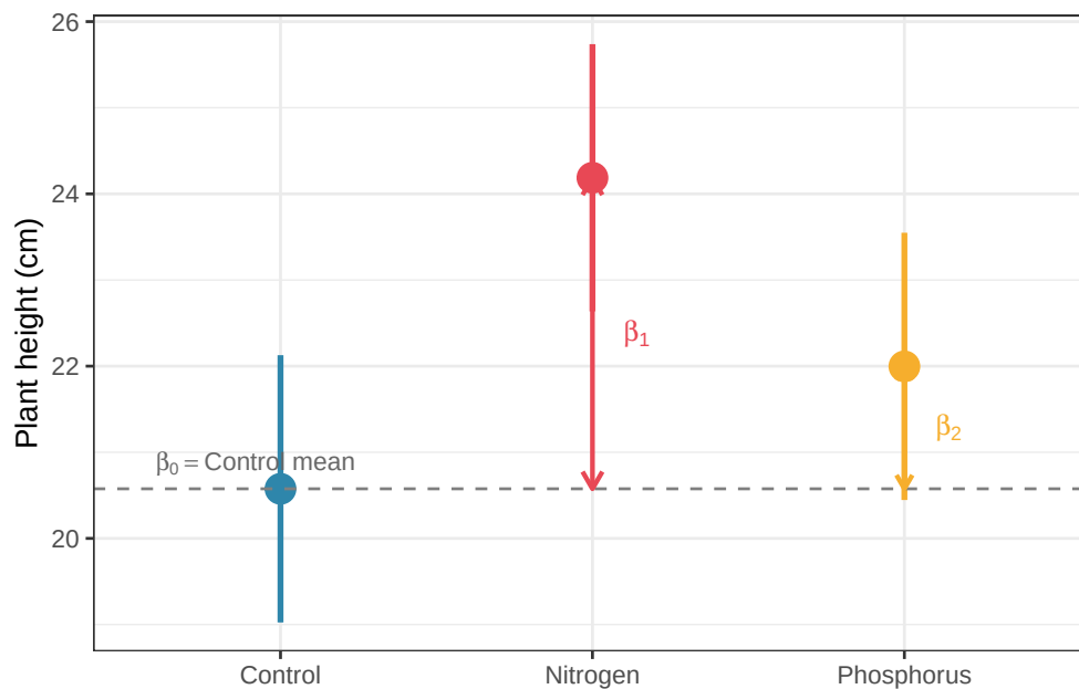
Figure 8.1.: The connection between regression coefficients and ANOVA group means under dummy coding. The intercept estimates the Control mean; the slope coefficients estimate the differences between each treatment group and the Control. Error bars show 95% confidence intervals for each group mean. Dashed line marks the Control mean (intercept)
