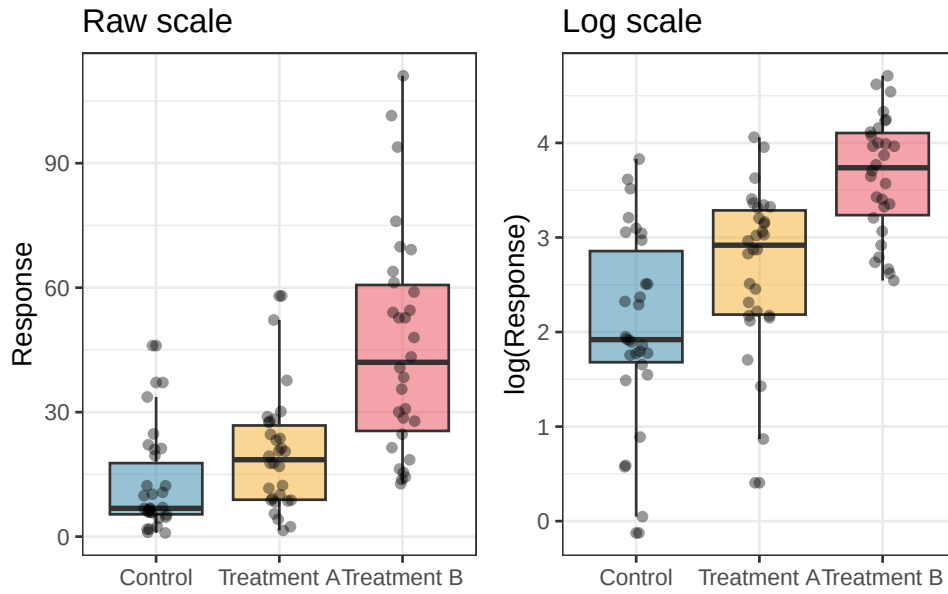
Figure 10.1.: Effect of log transformation on a right-skewed response. Left: raw counts with a long right tail and variance increasing with the mean. Right: log-transformed values with approximately symmetric distribution and homogeneous variance across groups. The log transformation is appropriate when within-group standard deviation is proportional to the group mean.
