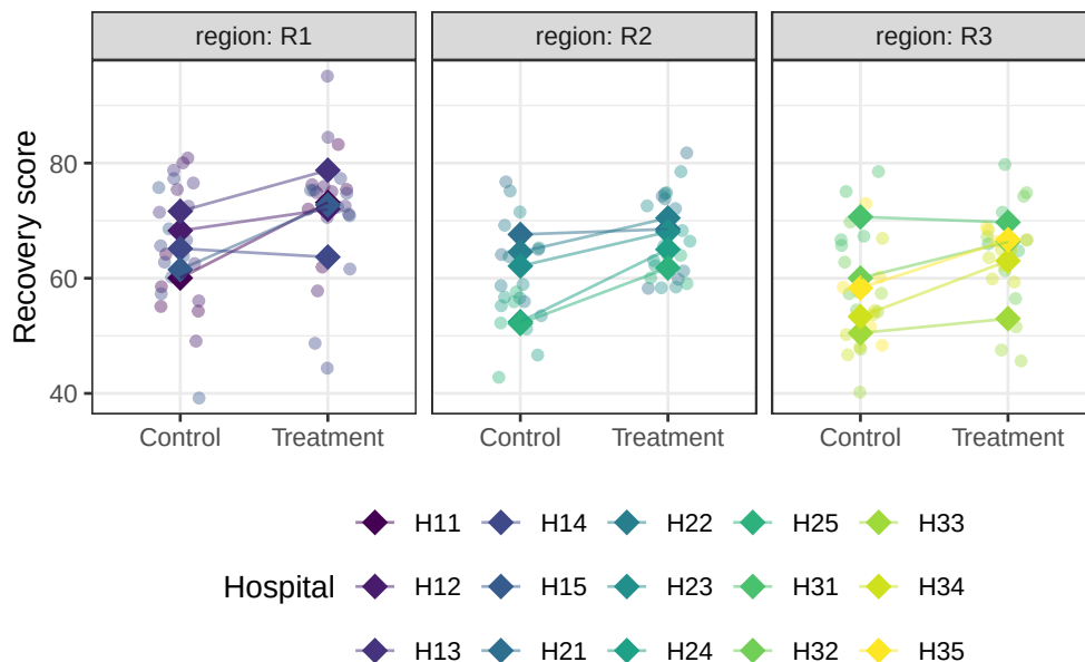
Figure 9.3.: Recovery scores by treatment group, hospital, and region. Each panel is a region; within each panel, points are coloured by hospital. The substantial variation in hospital means within and across regions illustrates why the nested random effect structure must be modelled explicitly.
