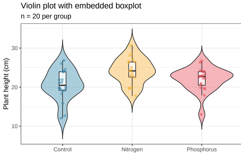
Figure 13.3.: Violin plot with embedded boxplot and individual observations for the fertiliser experiment. The violin shape shows the full distribution; the inner boxplot provides the summary statistics; the points show individual observations. This is the most complete single-panel display for group comparisons.
