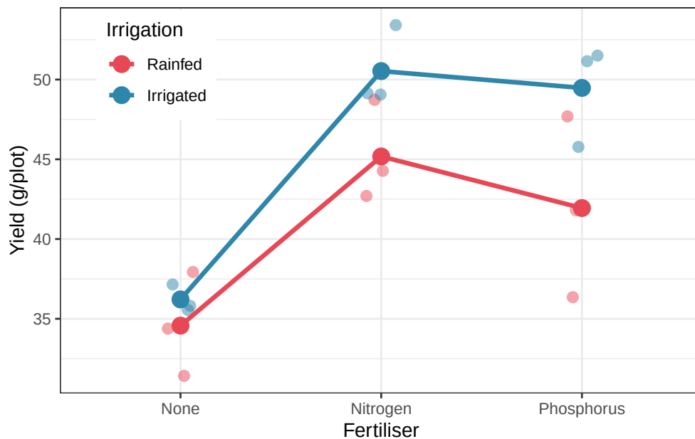
Figure 7.2.: Mean wheat yield by irrigation regime and fertiliser type in a split-plot design. Points show individual plot yields. Lines connect the means of each irrigation group across fertiliser types. The larger spread of the rainfed points reflects the greater whole-plot variability in unirrigated fields.
