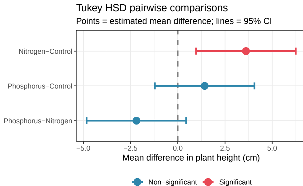
Figure 13.5.: Forest plot of Tukey HSD pairwise comparisons from the fertiliser experiment. Each row is one comparison; points show the estimated mean difference; horizontal lines show the 95% CI. The vertical dashed line at zero marks no difference, comparisons whose CI does not cross zero are significant after Tukey correction.
