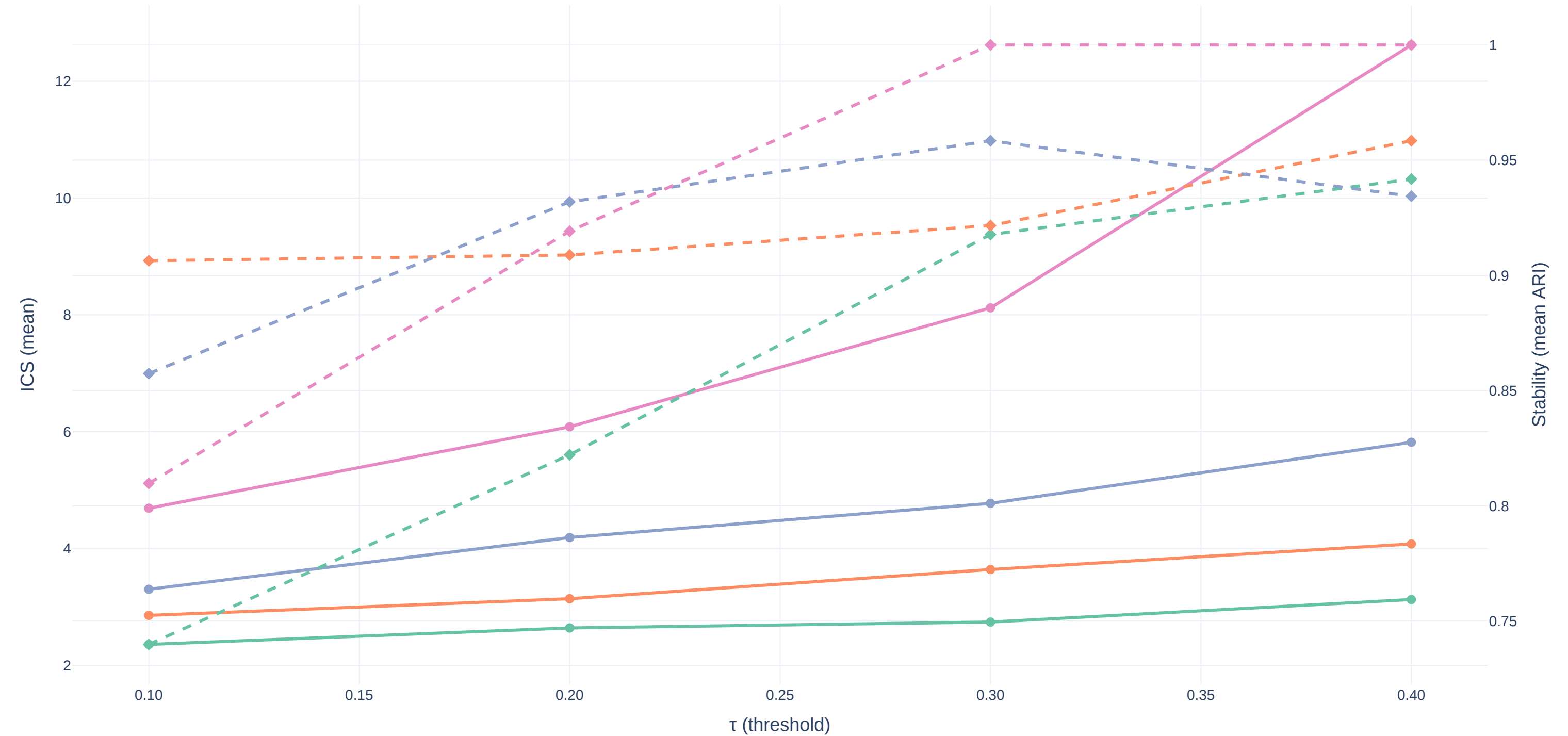
ICS & Stability vs \tau – Escherichia / Blood Culture
