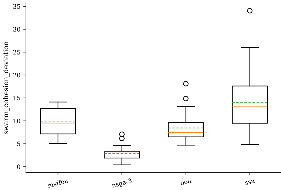
urban — swarm_cohesion_deviation
