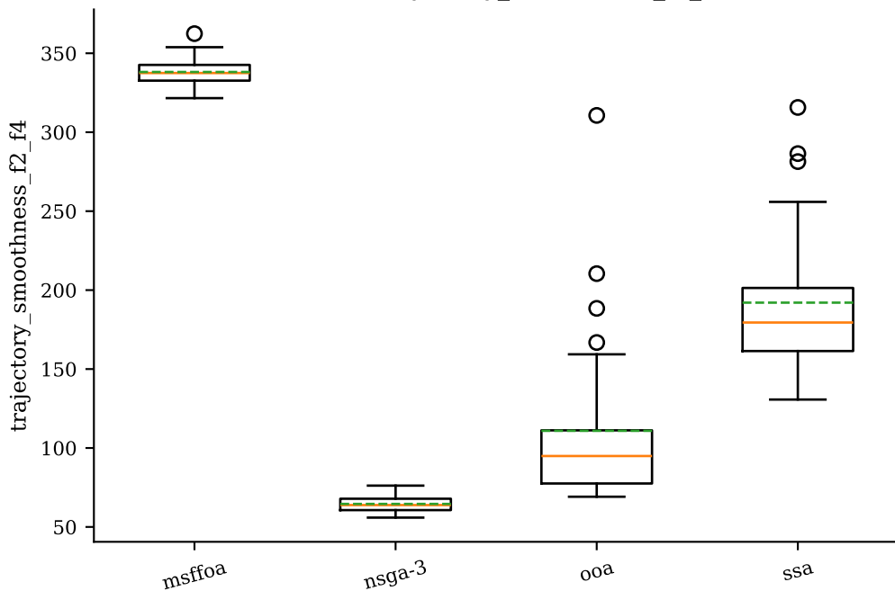
urban — trajectory_smoothness_f2_f4
