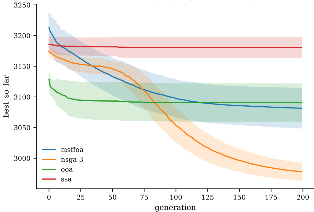
forest — best_so_far (lower=better)
