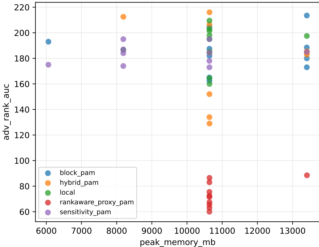
HM12 memory vs rank-AUC
