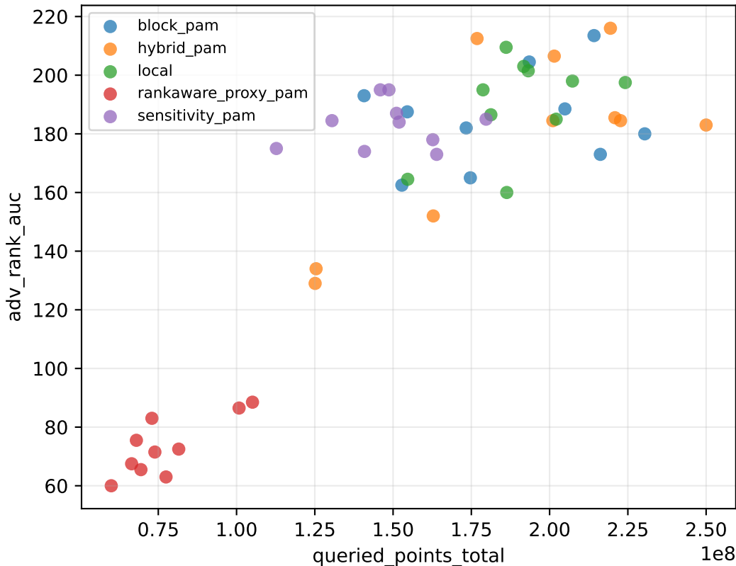
HM12 queries vs rank-AUC
