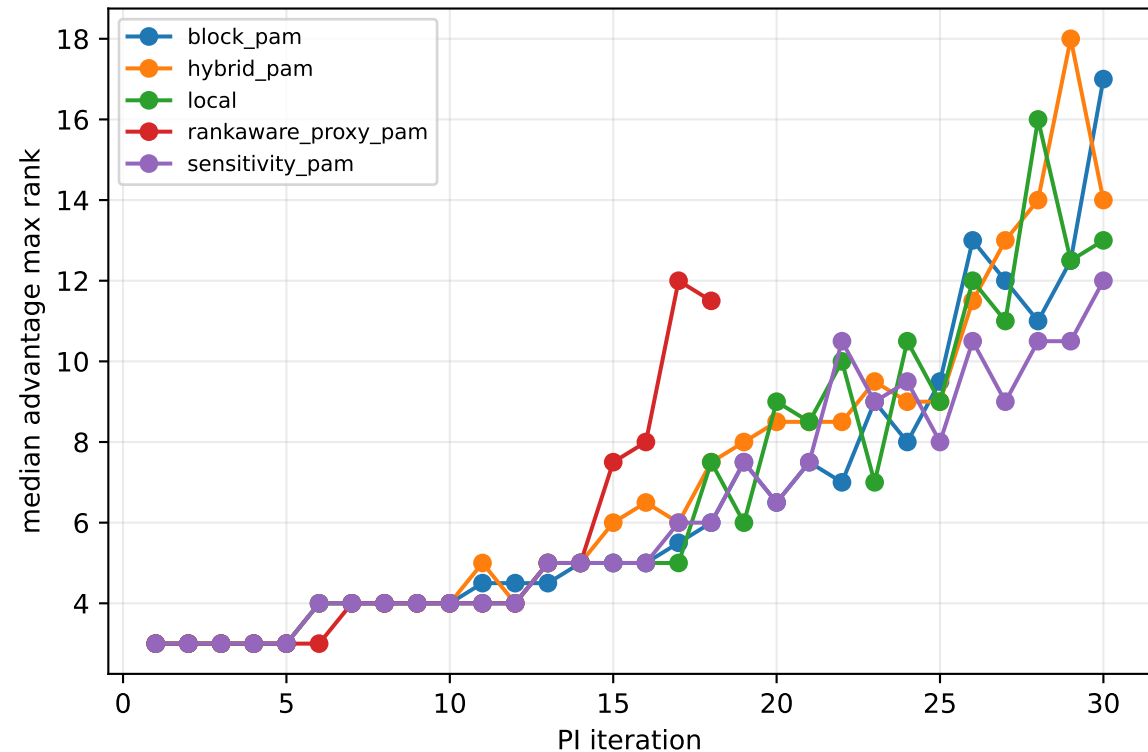
HM12 rank trajectory (typical seed 9)
