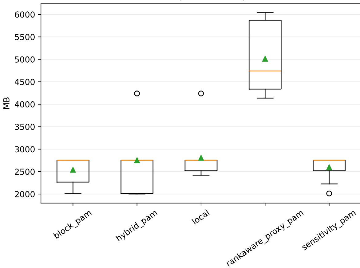
HM8 peak memory
