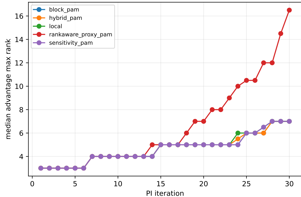
HM8 rank trajectory (typical seed 1)
