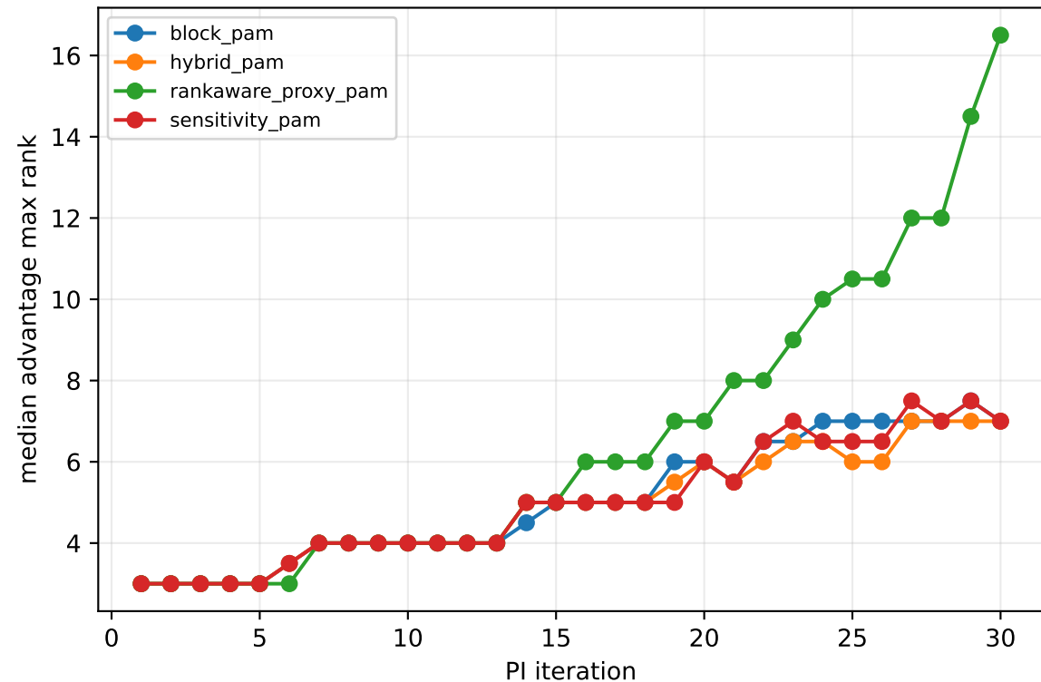
Rankaware vs baselines
