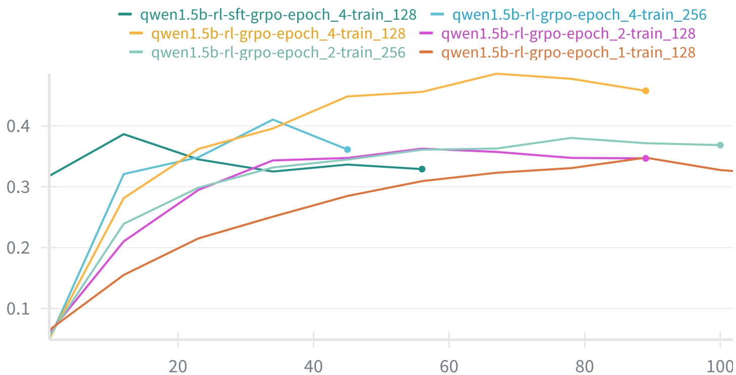
avg_reward
