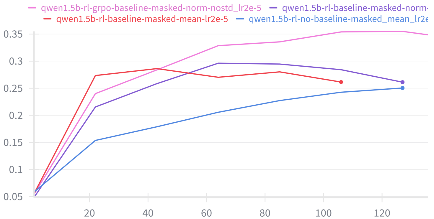
avg_reward
