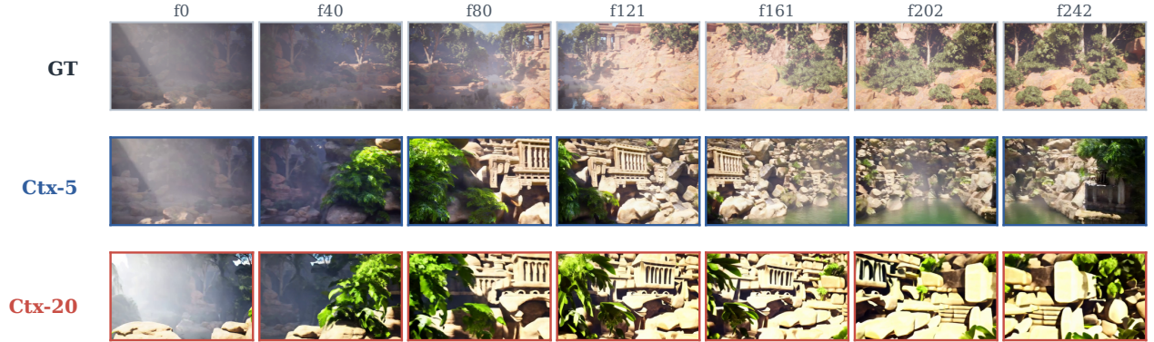
Figure 5 Replay progression on a fixed GT camera trajectory. The first row is the dataset trajectory; the remaining rows show generated replay frames from the Context K=5 and Context K=20 rows at matched time indices. This panel is a visual companion to the Replay PSNR/SSIM/LPIPS metrics, showing where background structure and object layout begin to drift across chunks.
