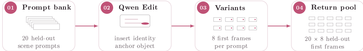
Figure 4 Qwen Edit construction of open-domain first frames. Each held-out environment prompt is edited into identity-anchored first frames, which seed the open-domain return probe.
