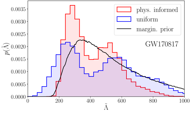
Figure 2. Marginalised posterior distributions of the tidal deformability \tilde{\Lambda} obtained from Bayesian parameter estimation for GW170817. The posterior using a physics-informed prior is shown in red, while the posterior using uniform priors from the LVK is shown in blue; we show the (marginalised) prior with the black curve. Note that the posterior from the LVK show support up to \tilde{\Lambda} = 2000 .
