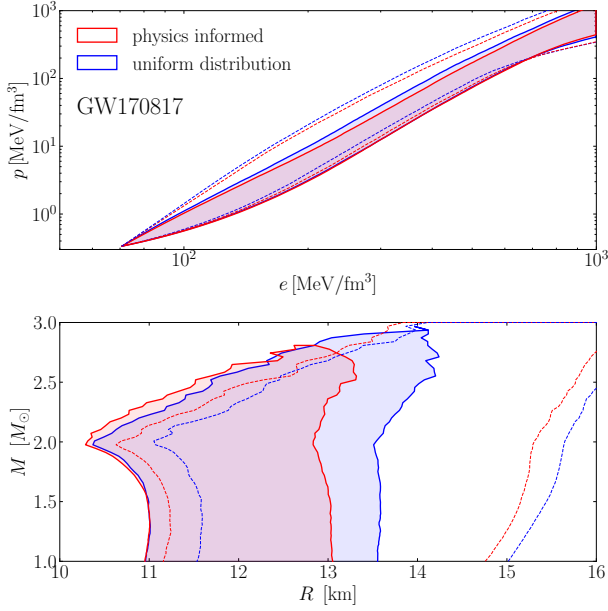
Figure 3. Posterior distributions of the cold nuclear EOS from analysis of GW170817 using the spectral parameterisation (Lindblom 2010). The top panel shows the posterior distributions in pressure–density space, while the bottom panel shows the reconstructed mass–radius curves. The shaded regions show the 90% credible intervals of the posterior distributions obtained from the analysis using the physics inspired priors (teal) and uniform priors (orange). The dashed curves show the 90% credible intervals of the effective priors, whilst the grey curve shows the 90% credible interval of the true distribution used to generate the priors.
