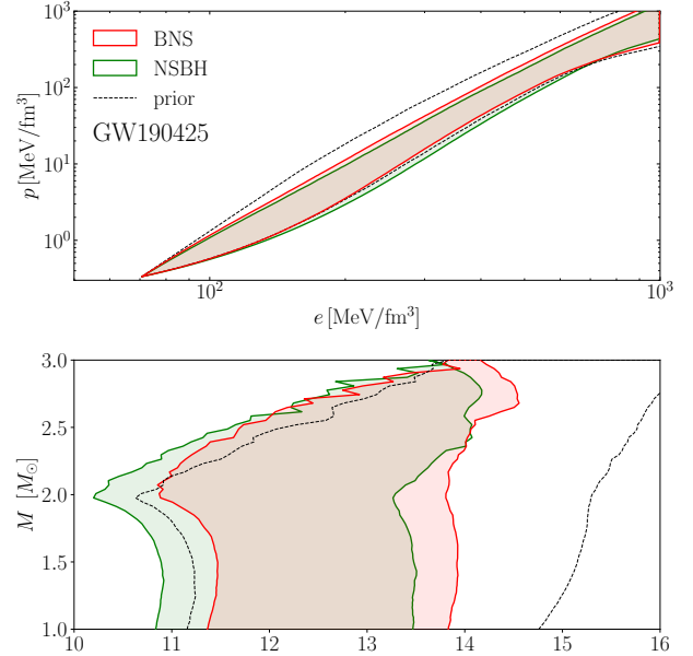
Figure 5. Posterior distributions of the cold nuclear EOS from analysis of GW190425 using the spectral parameterisation (Lindblom 2010). The top panel shows the posterior distributions in pressure–density space, while the bottom panel shows the reconstructed mass–radius curves. The shaded regions show the 90% credible intervals of the posterior distributions obtained from the analysis using the physics inspired BNS priors (teal) and the NSBH prior (orange). The black dashed curve shows the 90% credible intervals of the effective priors, whilst the grey curve shows the 90% credible interval of the true distribution used to generate the priors.
