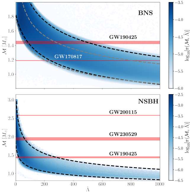
Figure 1. Priors for the source-frame chirp mass \mathcal{M} and the dimensionless tidal deformability \tilde{\Lambda} in the case of BNS (top panel) or NSBH binaries (bottom panel). In both panels, dashed black curves indicate analytic fits to the 90% contours of the distribution given in Equation (6), while the dashed gray curves are the corresponding fits obtained when imposing the GW170817 constraint on the prior following S. Altiparmak et al. (2022). Horizontal red bands represent the 90% credible intervals for the measured chirp masses of GW170817 (B. P. Abbott et al. 2017), GW190425 (B. P. Abbott et al. 2020), GW200115 (R. Abbott et al. 2021), and GW230529 (A. G. Abac et al. 2024).
