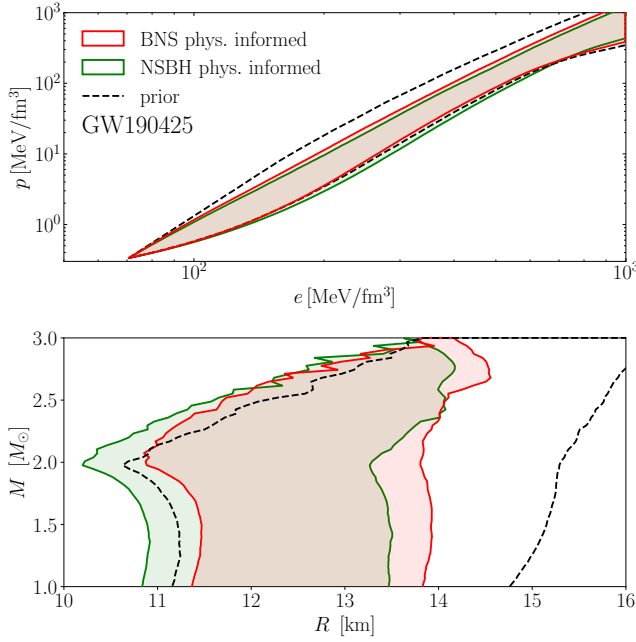
Figure 5. The same as in Figure 3 but for the GW190425 event. The top panel shows the posterior distributions in pressure–density space, while the bottom panel shows the reconstructed mass–radius curves. The shaded regions show the 90% credible intervals of the posterior distributions obtained from the analysis using the physics-informed BNS prior (red) and the NSBH prior (green). The black dashed curve shows the 90% credible interval of the effective prior of the relationship between chirp mass and tidal deformability for the physics-informed prior, when mapped to the spectral parameterization.
