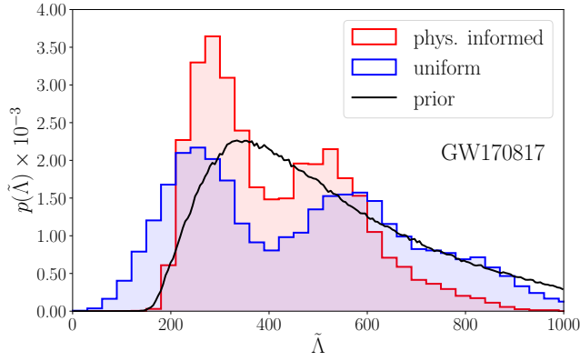
Figure 2. Marginalized posterior distributions of the tidal deformability \tilde{\Lambda} for GW170817. The posterior using a physics-informed prior is shown in red, while the posterior using uniform priors from the LVK analysis is shown in blue; we show the (marginalized) prior with the black curve. Note that the posterior from the LVK shows support up to \tilde{\Lambda} = 2000 .
