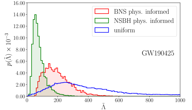
Figure 4. The same as in Figure 2 but for the GW190425 event. The posterior using a physics-informed prior for BNS mergers is shown in red, while the posterior for NSBH mergers is shown in green. The posterior using uniform priors and assuming a BNS origin from the LVK is reported in blue.
