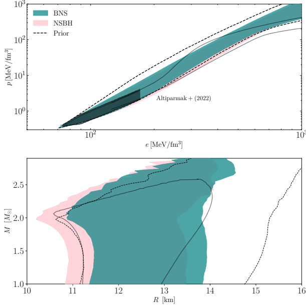
Figure 5. Posterior distributions of the cold nuclear equation of state from analysis of GW190425 using the spectral parameterisation (Lindblom 2010). The top panel shows the posterior distributions in pressure–density space, while the bottom panel shows the reconstructed mass–radius curves. The shaded regions show the 90% credible intervals of the posterior distributions obtained from the analysis using the physics inspired BNS priors (teal) and the NSBH prior (orange). The black dashed curve shows the 90% credible intervals of the effective priors, whilst the grey curve shows the 90% credible interval of the true distribution used to generate the priors.
