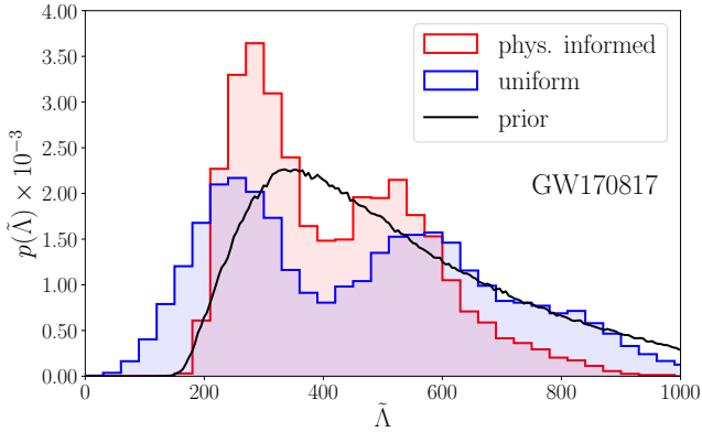
Figure 2. Marginalised posterior distributions of the tidal deformability \tilde{\Lambda} for GW170817. The posterior using a physics-informed prior is shown in red, while the posterior using uniform priors from the LVK analysis is shown in blue: we show the (marginalised) prior with the black curve. Note that the posterior from the LVK shows support up to \tilde{\Lambda} = 2000 .
