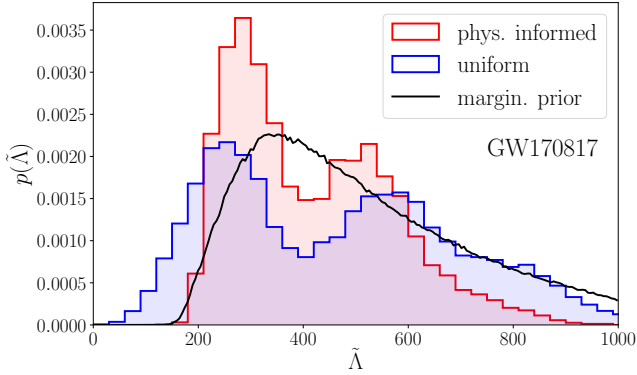
Figure 2. Marginalised posterior distributions of the tidal deformability \tilde{\Lambda} obtained from Bayesian parameter estimation for GW170817. The posterior using a physics-informed prior is shown in red, while the posterior using uniform priors from the LVK is shown in blue; we show the (marginalised) prior with the black curve. Note that the posterior from the LVK show support up to \tilde{\Lambda} = 2000 .
