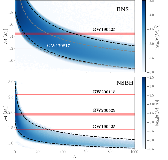
Figure 1. Priors for the source-frame chirp mass \mathcal{M} and the dimensionless tidal deformability \tilde{\Lambda} in the case of BNSs (top panel) or NSBH binaries (bottom panel). In both panels, dashed black lines indicate analytic fits to the 90% contours of the distribution given in Eq. (6), while the dashed grey lines are the corresponding fits obtained when imposing the GW170817 constraint on the prior, following (Altiparmak et al. 2022). Horizontal red bands represent the 90% credible intervals for the measured chirp masses of GW170817 (Abbott et al. 2017), GW190425 (Abbott et al. 2020), GW200115 (Abbott et al. 2021), and GW230529 (Abac et al. 2024).
