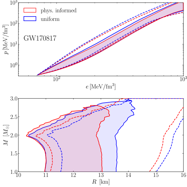
Figure 3. Posterior distributions of the range of pressures and energy densities for a nuclear-matter EOS (top panel) and of the corresponding masses and radii (bottom panel) in the case of GW170817. In both panels, the shaded regions show the 90% credible intervals of the posterior distributions obtained using the physics-informed priors (red) or the uniform priors (blue), while the dashed curves show the 90% credible intervals of the effective priors of the relationship between chirp mass and tidal deformability for the uniform (blue) and physics-informed (red) priors, when mapped to the spectral parameterisation.
