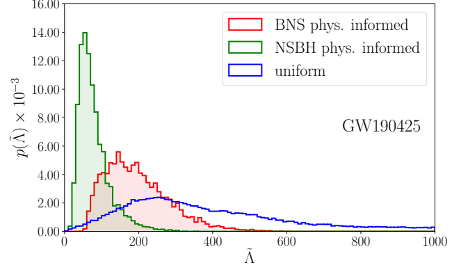
Figure 4. The same as in Fig. 2 but for the GW190425 event. The posterior using a physics-informed prior for BNS mergers is shown in red, while the posterior for NSBH mergers is shown in green. The posterior using uniform priors and assuming a BNS origin from the LVK is reported in blue.
