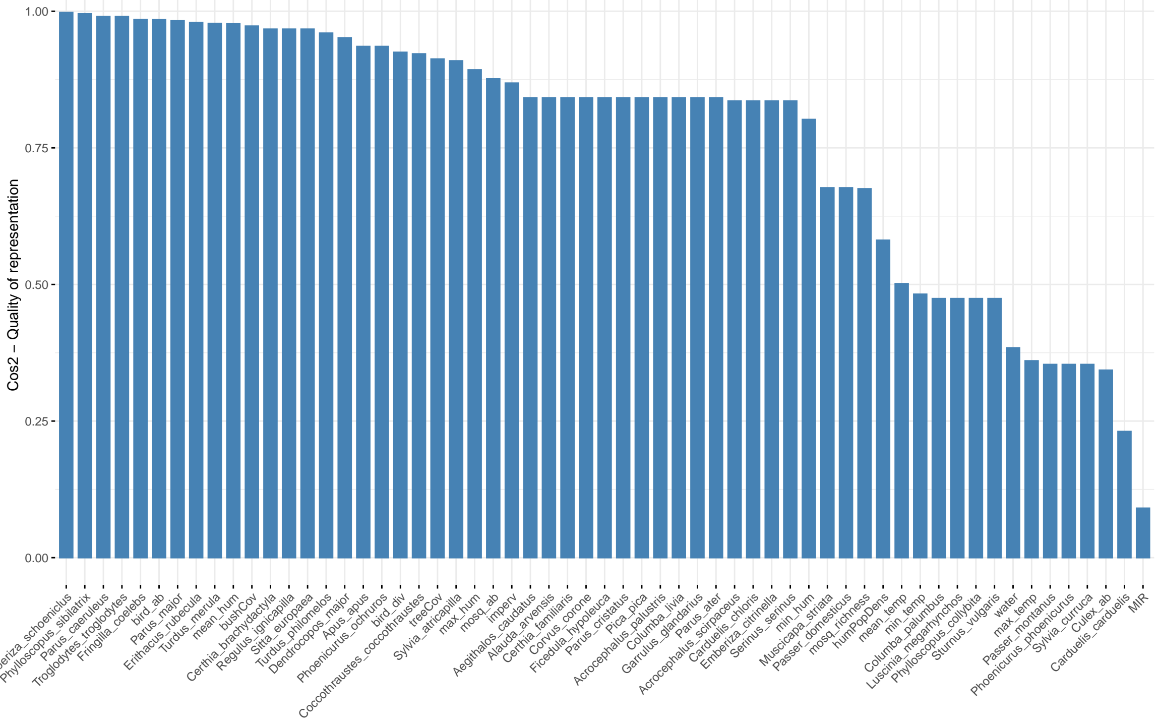
Cos2 of variables to Dim-1-2
