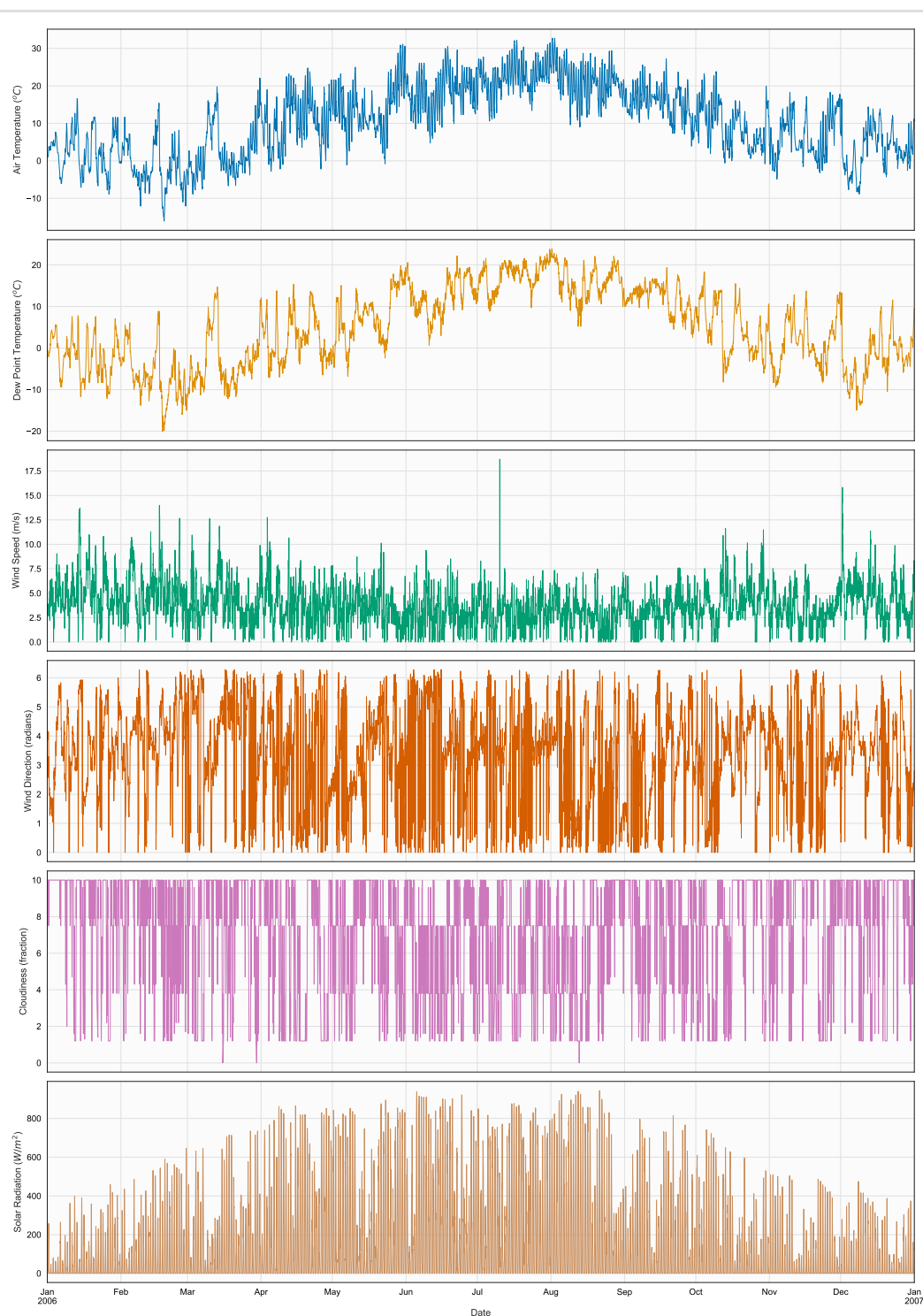
Figure 2. Time series of MET, WB2, in file 2006_Met1.npt
