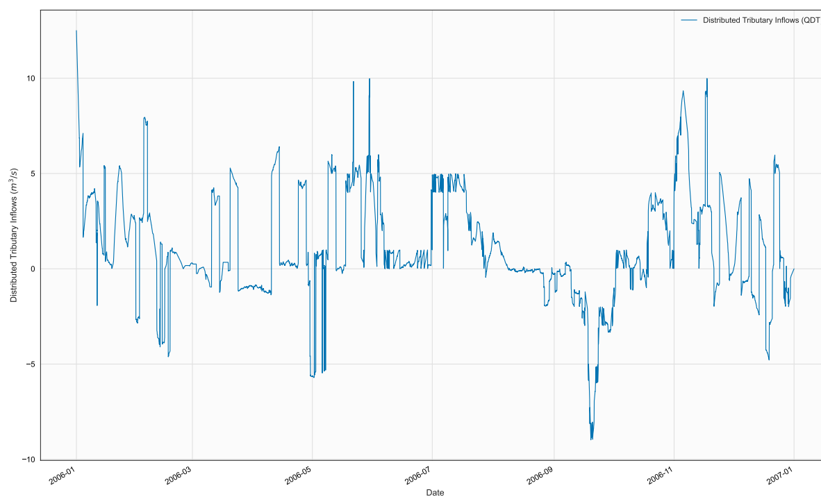
Figure 26. Time series of QDT, BR5, in file 2006_Mqwb_72smooth.npt
