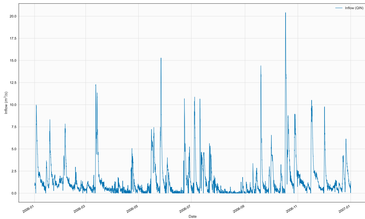
Figure 3. Time series of QIN, BR1, in file 2006_DeerCrk_Qin.npt
