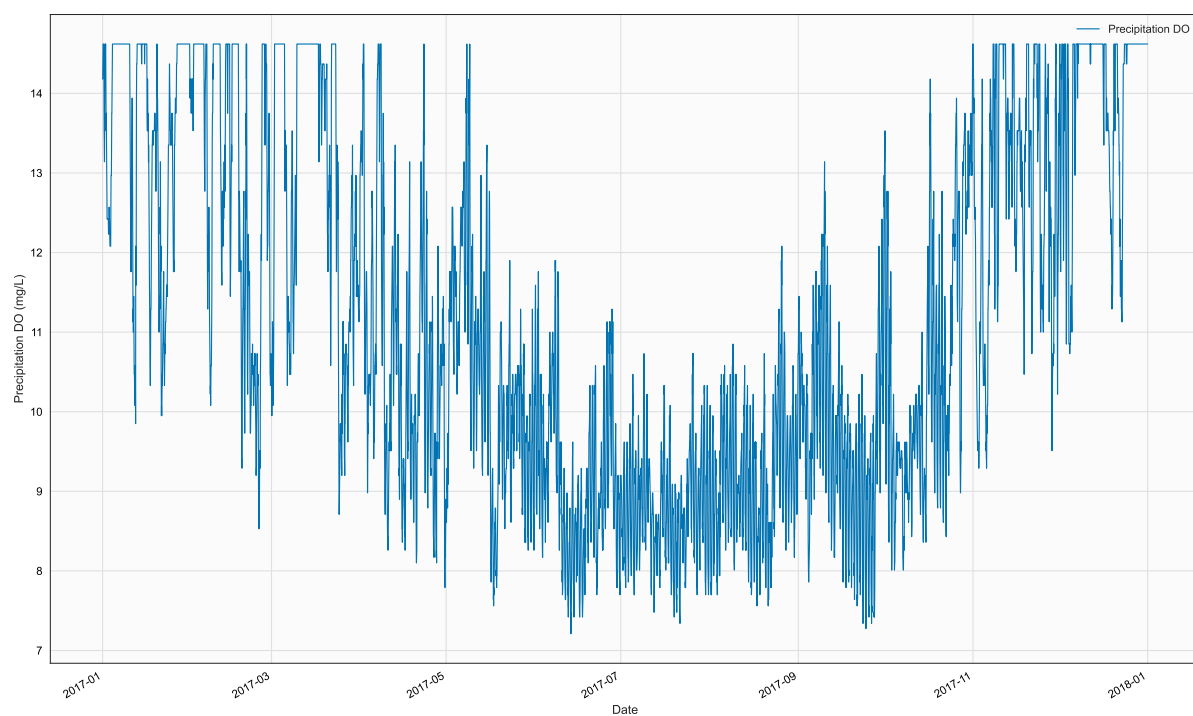
Figure 41. Time series of CPR, BR1, in file 2017_Pre_DO.npt
