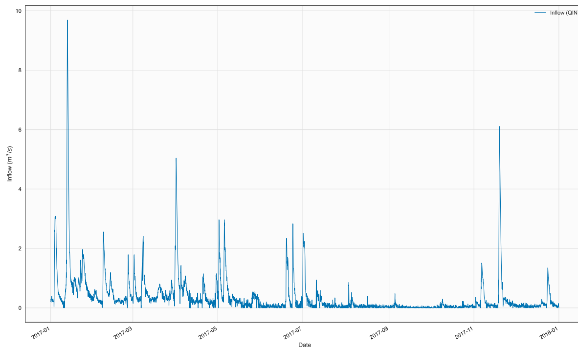
Figure 5. Time series of QIN, BR3, in file 2017_IslandCrk_Qin.npt
