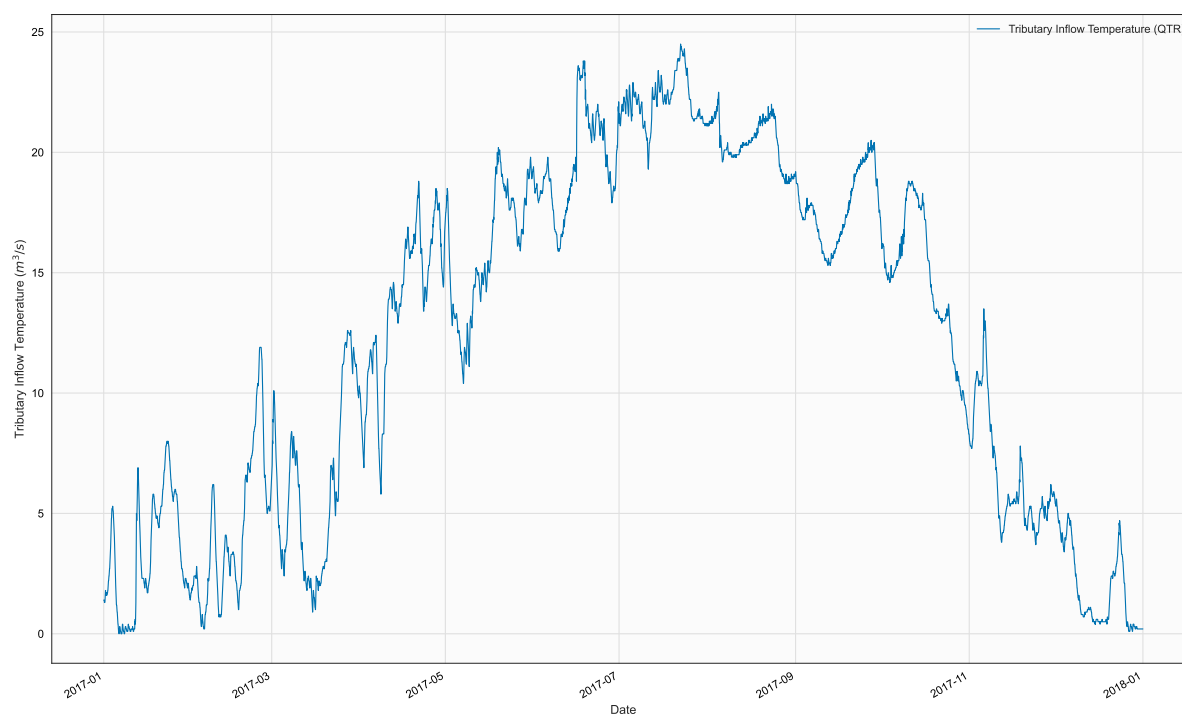
Figure 21. Time series of TTR, TR3, in file 2017_MahoningR_Ttr.npt
