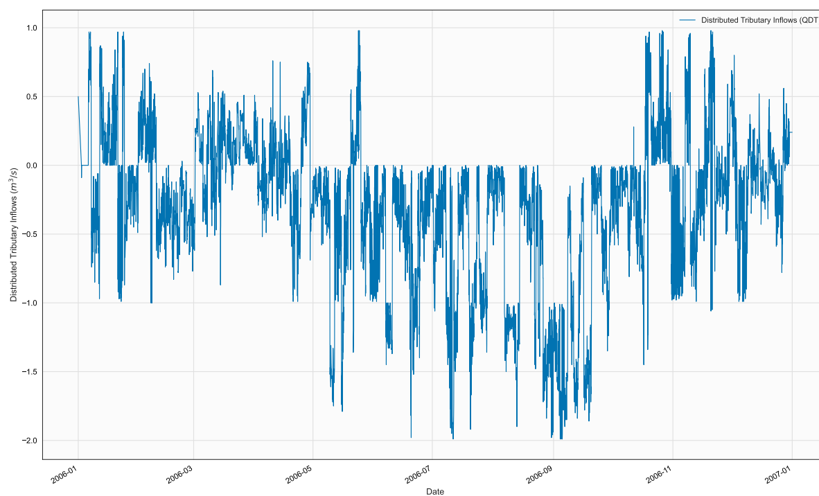
Figure 22. Time series of QDT, BR1, in file 2006_Kqwb_72hsmooth.npt
