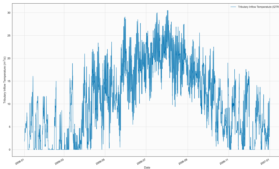
Figure 16. Time series of TTR, TR1, in file 2006_Tin_WestBranch_est3.npt
