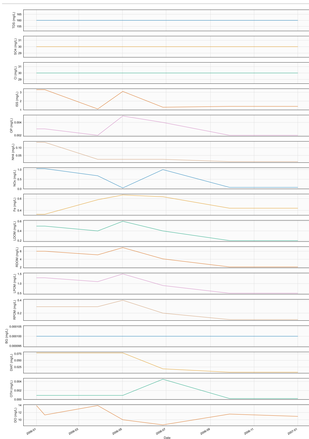
Figure 24. Time series of CDT, BR1, in file 2006_CDT1.npt
