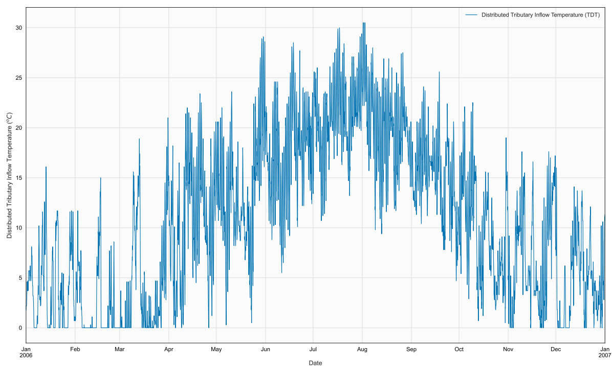
Figure 23. Time series of TDT, BR1, in file 2006_Tdt.npt
