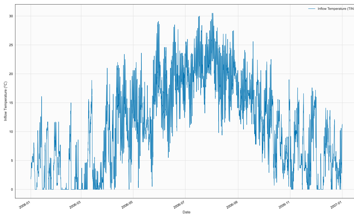
Figure 6. Time series of TIN, BR2, in file 2006_Tin_WestBranch_est1.npt
