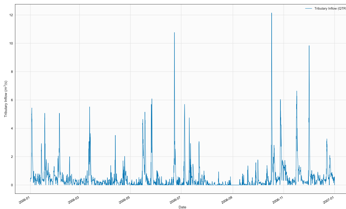
Figure 15. Time series of QTR, TR3, in file 2006_Qtr_Hinkley.npt
