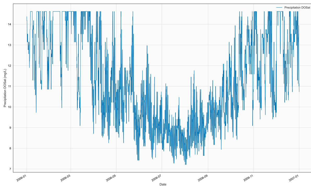
Figure 31. Time series of CPR, BR1, in file 2006_Pre_DO.npt
