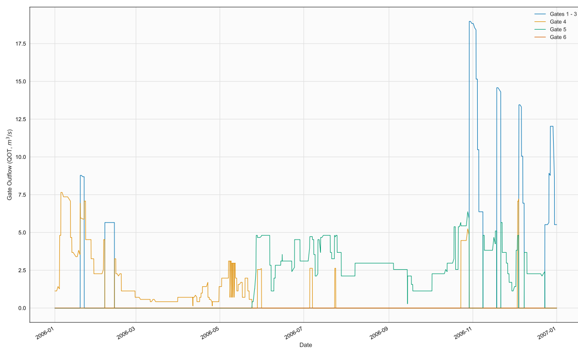
Figure 12. Time series of QGT, in file 2006_MJKirwanDam.npt
