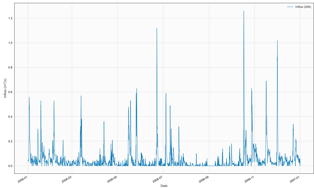
Figure 4. Time series of QIN, BR3, in file 2006_Qin_noname.npt
