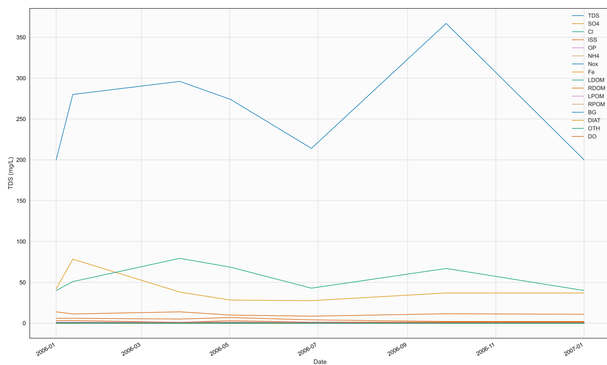
Figure 10. Time series of CIN, BR3, in file 2006_Cin_nonameEst.npt
