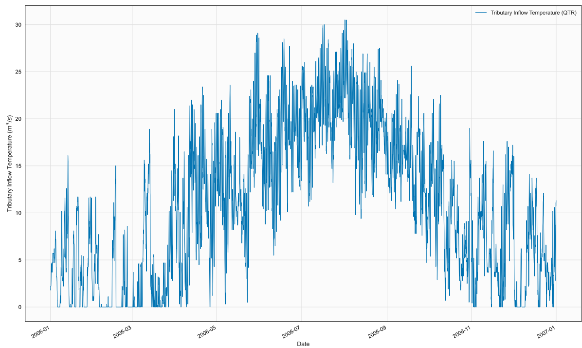
Figure 18. Time series of TTR, TR3, in file 2006_Tin_WestBranch_est5.npt
