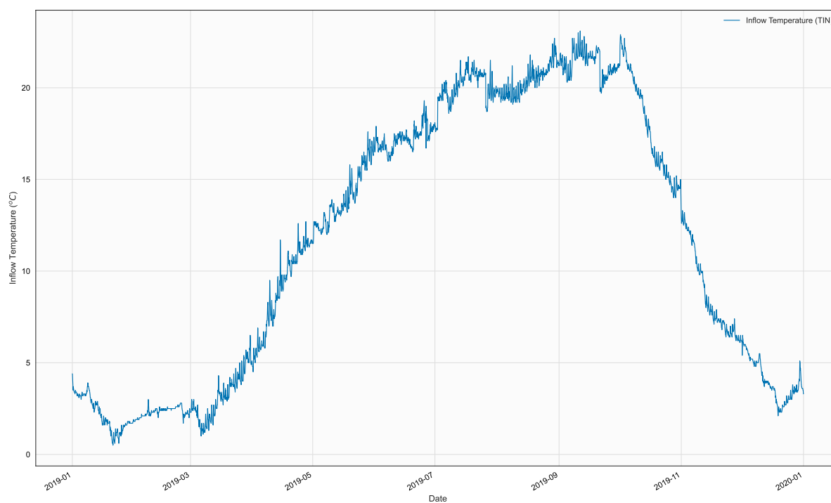
Figure 16. Time series of TIN, BR3, in file 2019_MJKirwan_Ttr.npt
