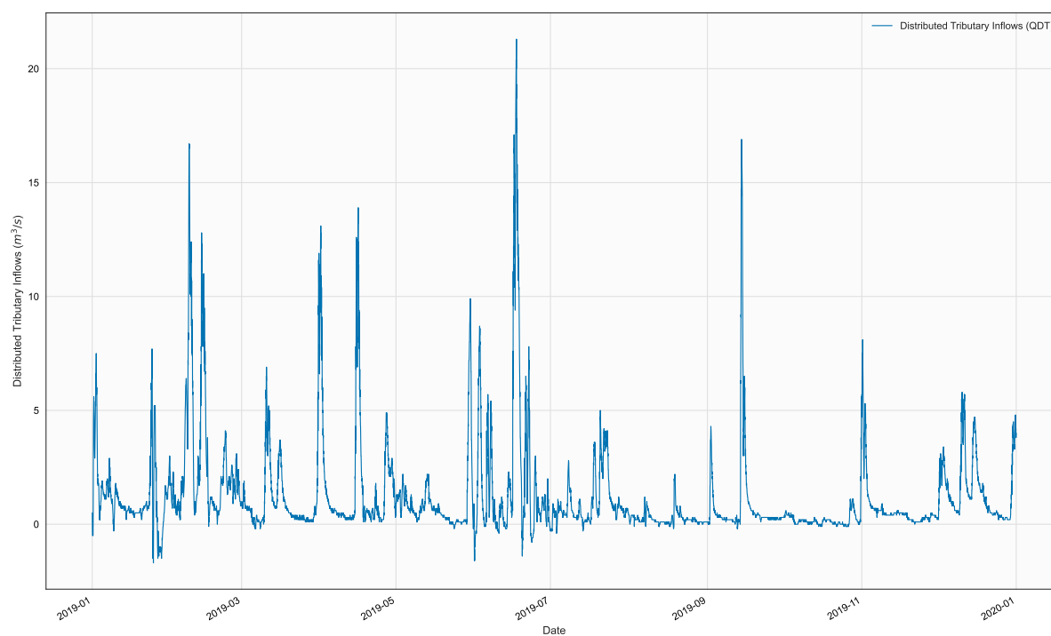
Figure 91. Time series of QDT, BR1, in file 2019_qdt_up1.npt
