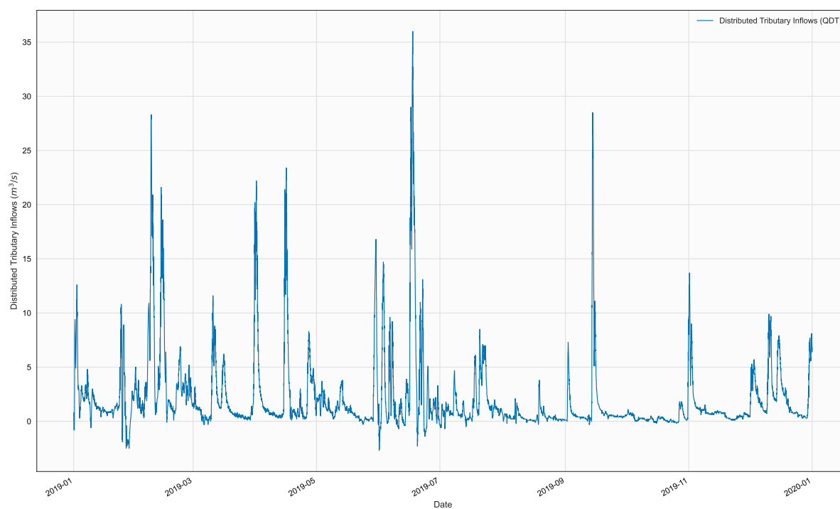
Figure 92. Time series of QDT, BR2, in file 2019_qdt_up2.npt
