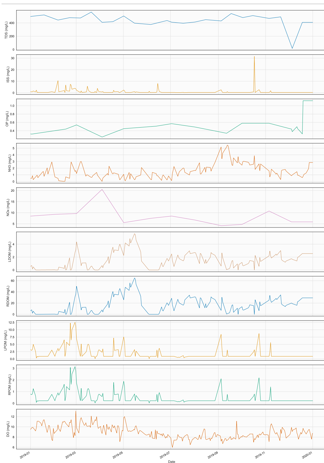
Figure 89. Time series of CTR, TR23, in file 2019_CampbellWwtp_Ctr.npt
