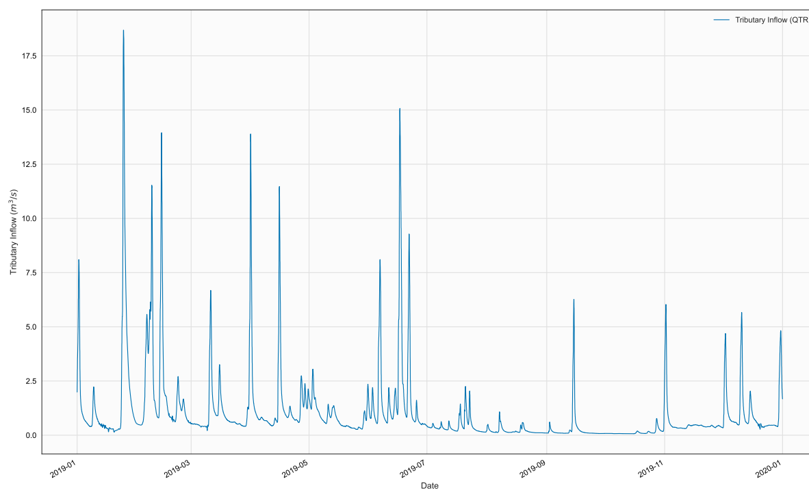
Figure 37. Time series of QTR, TR19, in file 2019_CrabCrk_Qtr_est15.npt
