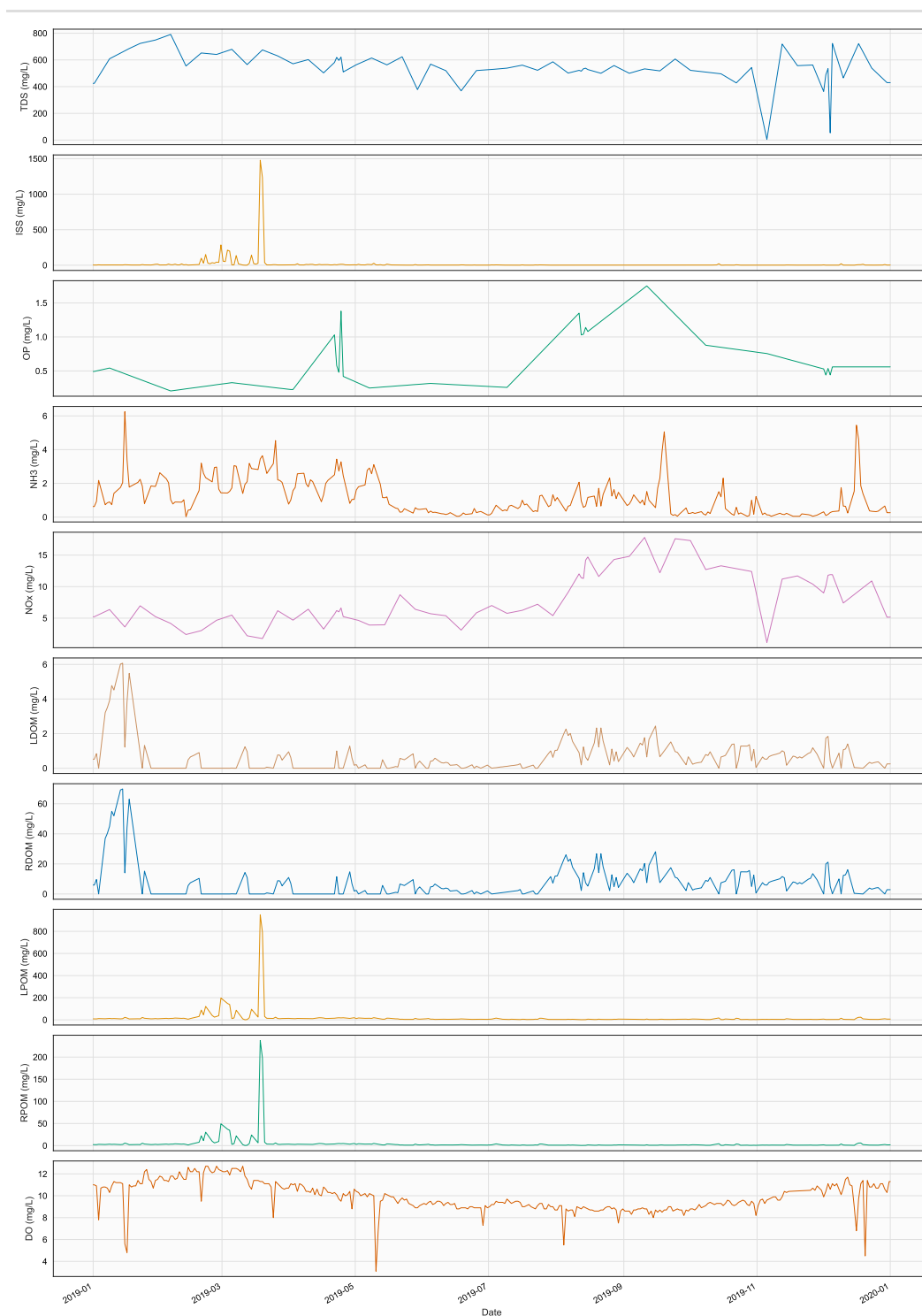
Figure 86. Time series of CTR, TR20, in file 2019_YoungsWwtp_Ctr.npt
