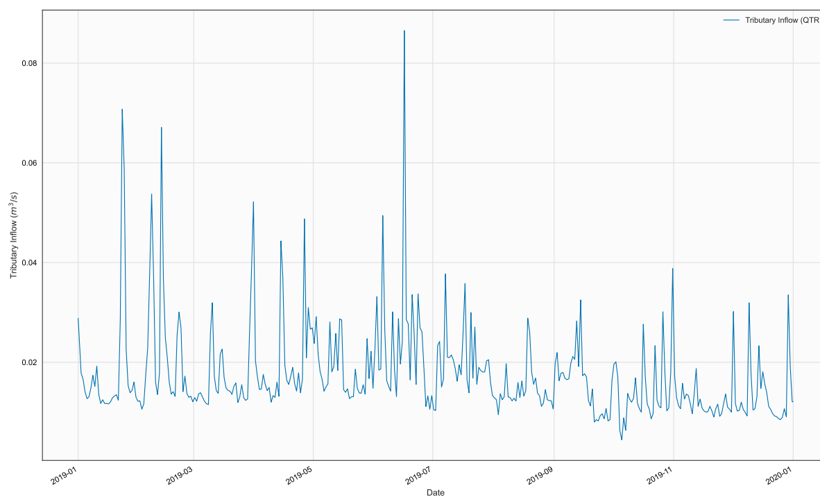
Figure 23. Time series of QTR, TR5, in file 2019_ThomasStrip_Qtr.npt
