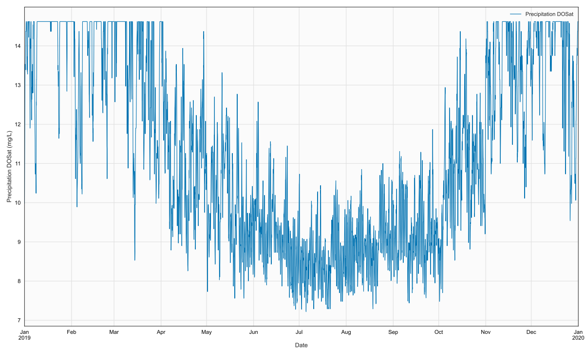
Figure 142. Time series of CPR, BR12, in file 2019_Pre_DO11.npt
