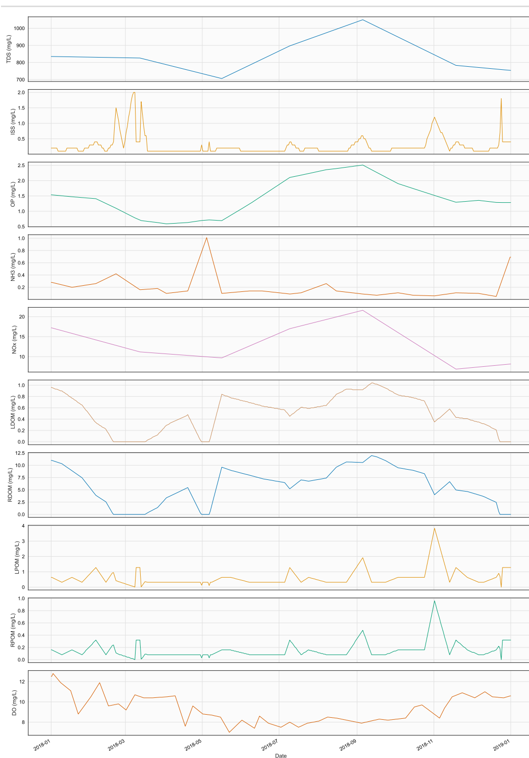
Figure 13. Time series of CTR, TR1, in file 2018_MeccaWwtp_Ctr.npt
