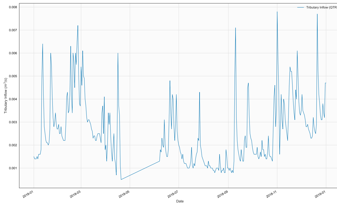
Figure 7. Time series of QTR, TR1, in file 2018_MeccaWwtp_Qtr.npt
