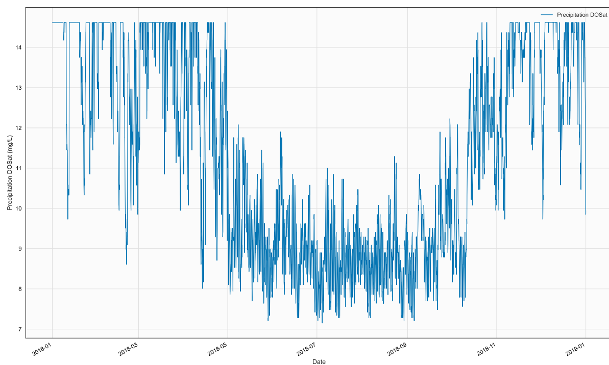
Figure 21. Time series of CPR, BR1, in file 2018_Pre_DO.npt
