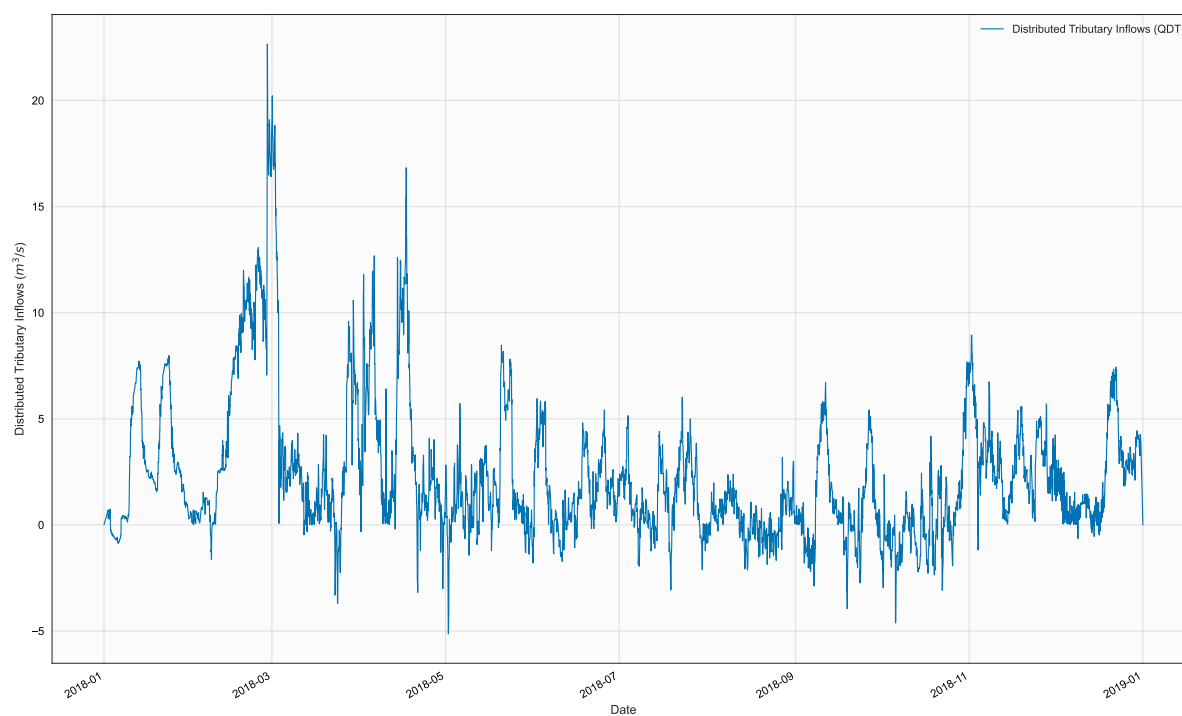
Figure 16. Time series of QDT, BR1, in file qwb_2_72hsm.npt
