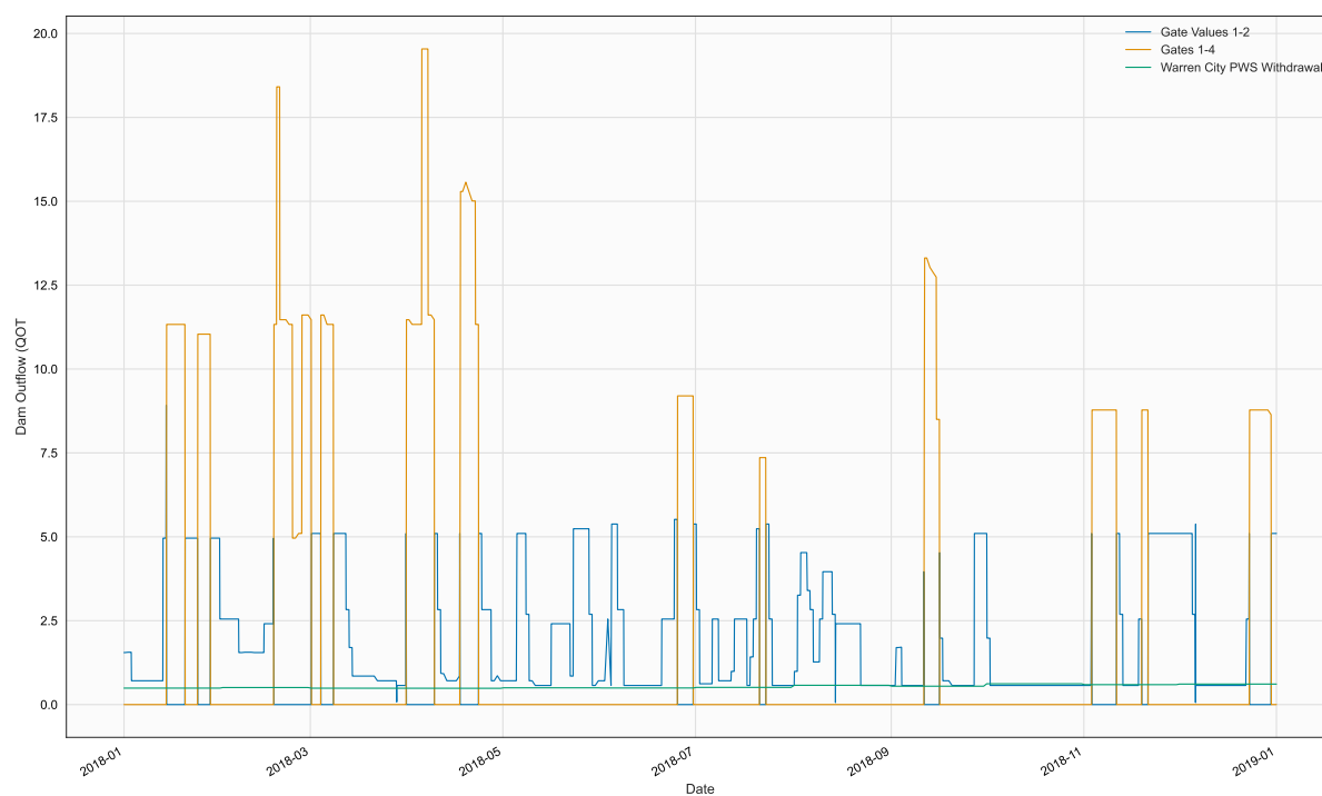
Figure 6. Time series of QOT, BR1, in file 2018_MosquitoDam.npt
