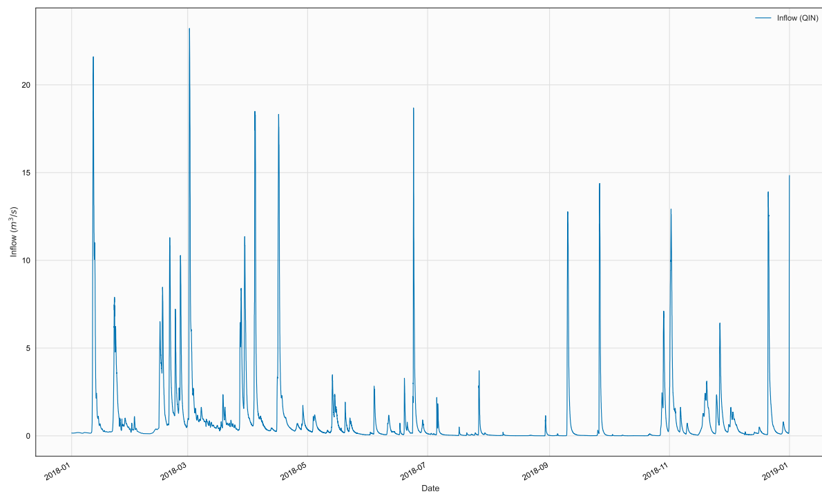
Figure 2. Time series of QIN, BR1, in file 2018_MosquitoCrk_Qin.npt
