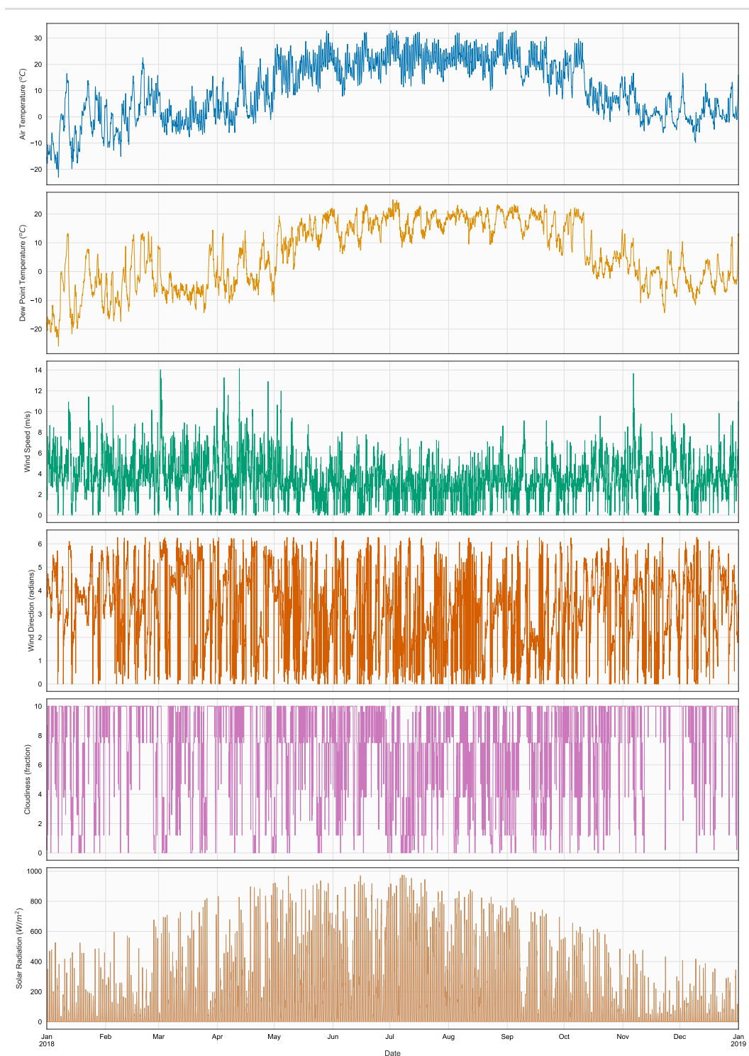
Figure 1. Time series of MET, WB1, in file 2018_Met.npt
