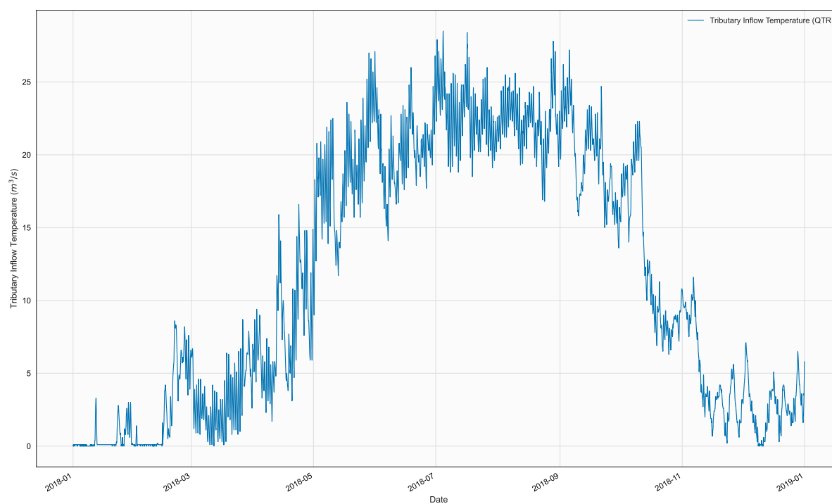
Figure 12. Time series of TTR, TR3, in file 2018_MosquitoCrk_Tin1.npt
