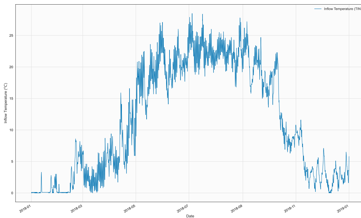
Figure 3. Time series of TIN, BR1, in file 2018_MosquitoCrk_Tin.npt
