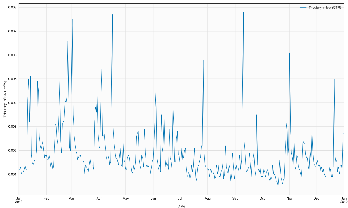
Figure 8. Time series of QTR, TR2, in file 2018_BazettaWwtp_Qtr.npt
