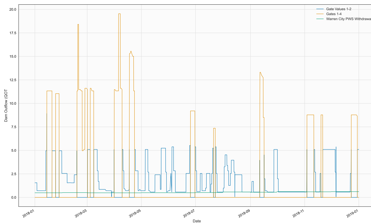
Figure 5. Time series of QGT, BR1, in file 2018_MosquitoDam.npt
