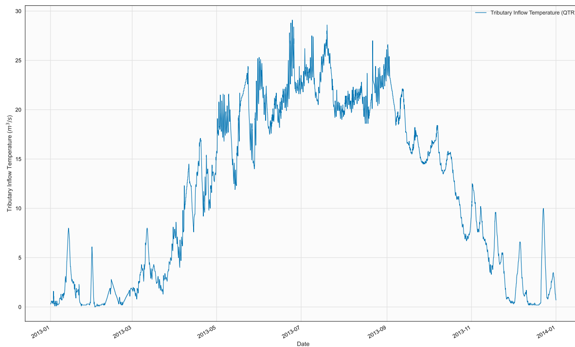
Figure 21. Time series of TTR, TR1, in file 2013_MahoningR_Tin4.npt
