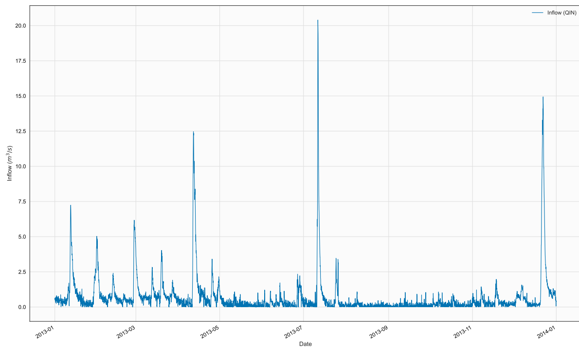
Figure 6. Time series of QIN, BR4, in file 2013_MillCrk_Qin.npt
