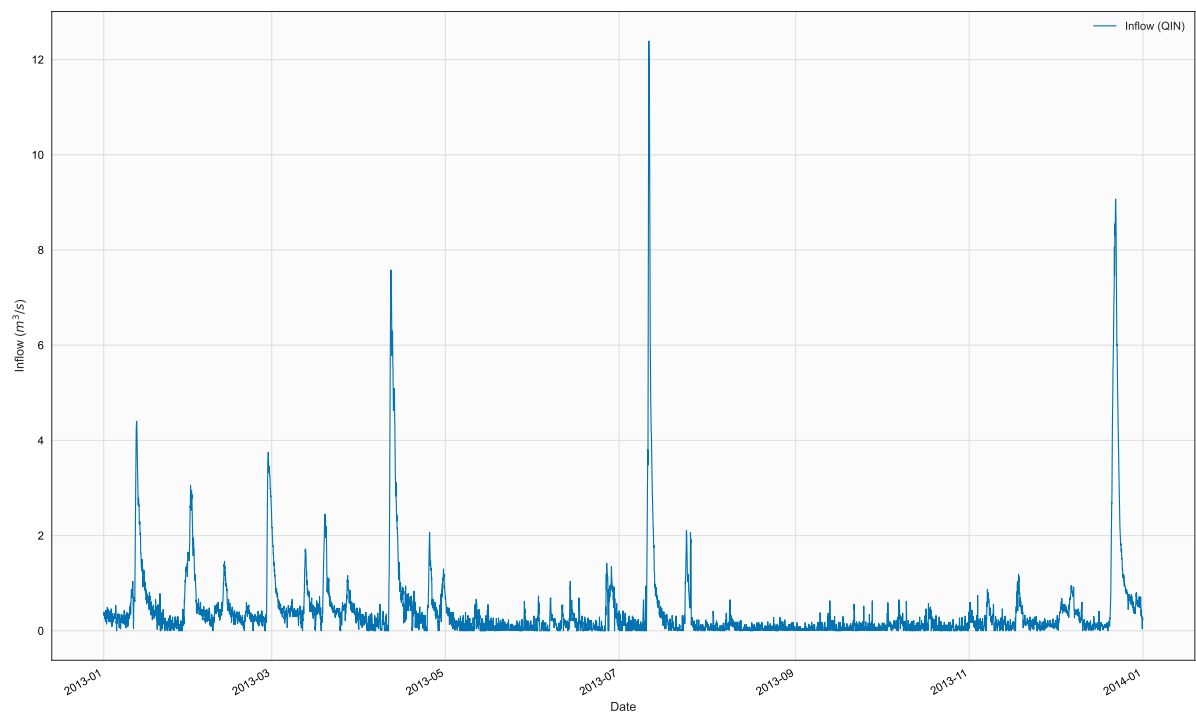
Figure 4. Time series of QIN, BR2, in file 2013_WillowCrk_Qin.npt
