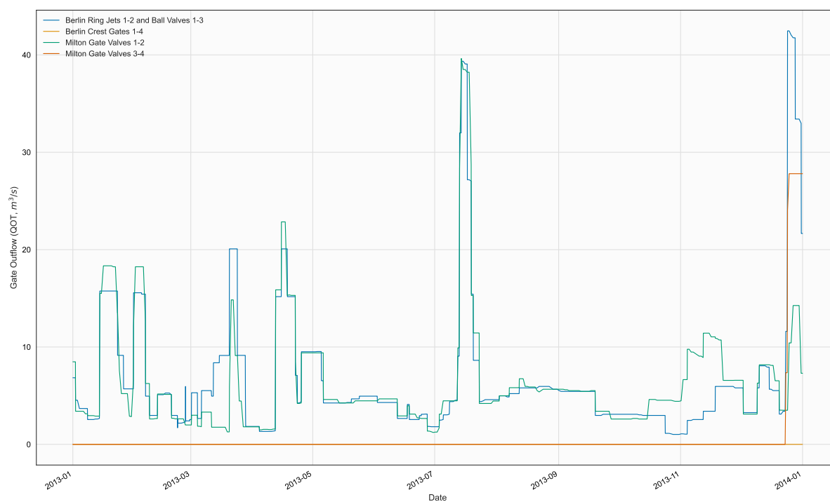
Figure 17. Time series of QGT, in file 2013_Ber_Mil_Dam.npt
