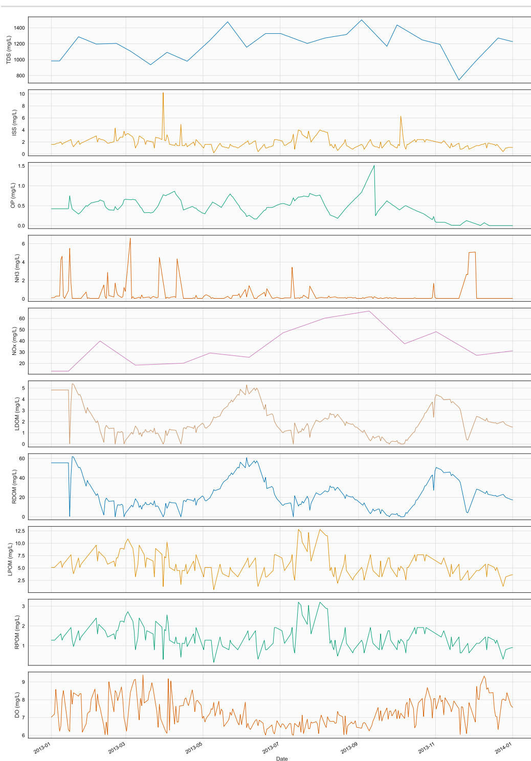
Figure 25. Time series of CTR, TR2, in file 2013_AllianceWwtp_Ctr.npt
