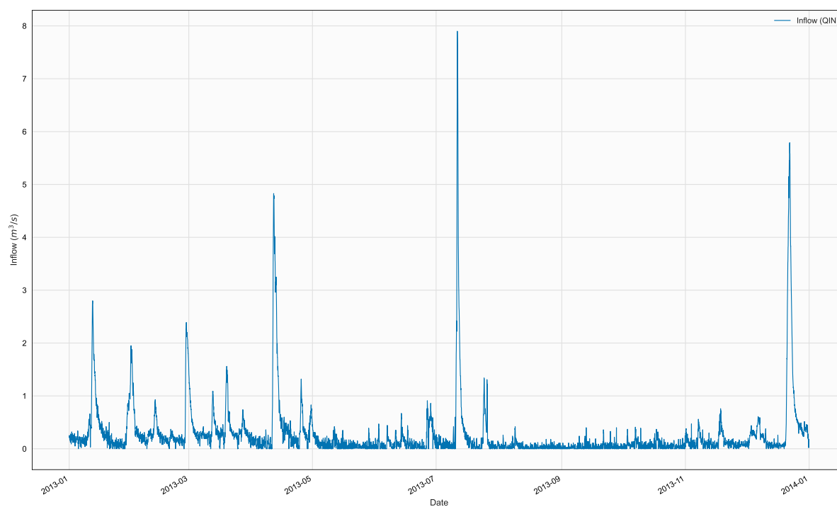
Figure 5. Time series of QIN, BR3, in file 2013_IslandCrk_Qin.npt
