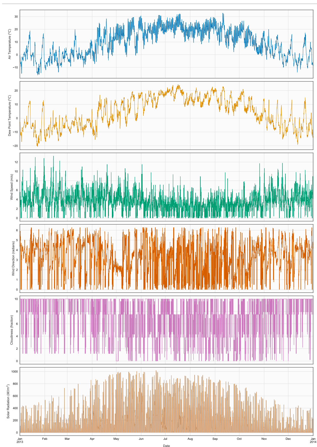
Figure 2. Time series of MET, WB2, in file 2013_Met1.npt
