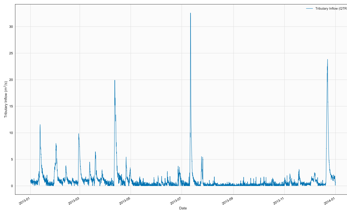
Figure 18. Time series of QTR, TR1, in file 2013_BeechCrk_Qtr.npt
