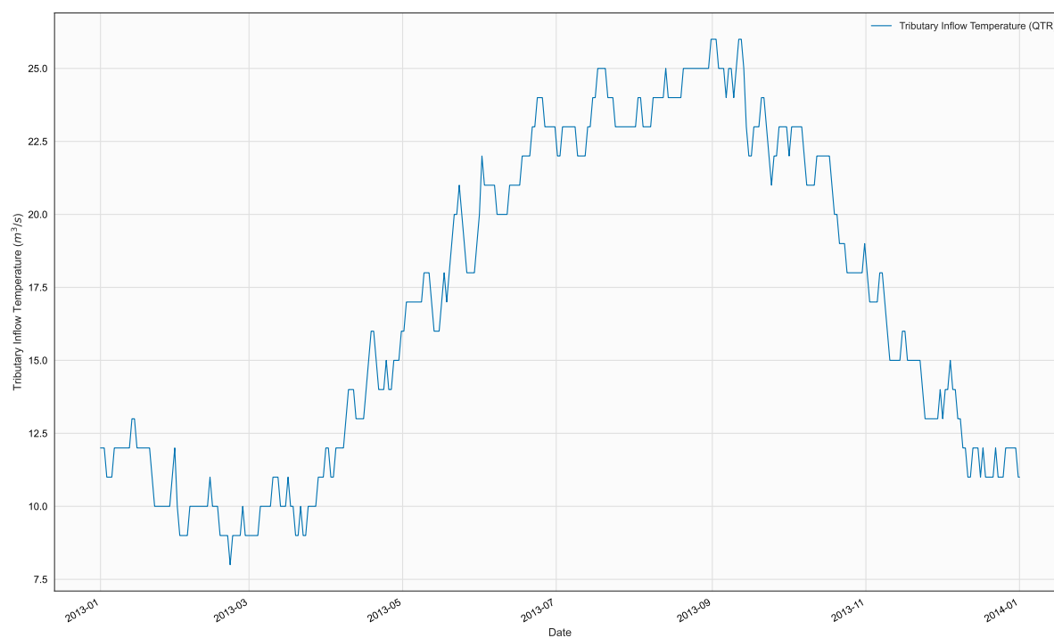
Figure 22. Time series of TTR, TR2, in file 2013_AllianceWwtp_Ttr.npt
