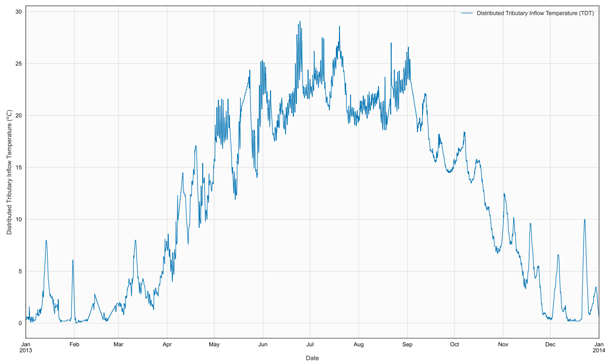
Figure 30. Time series of TDT, BR5, in file Mtdt.npt
