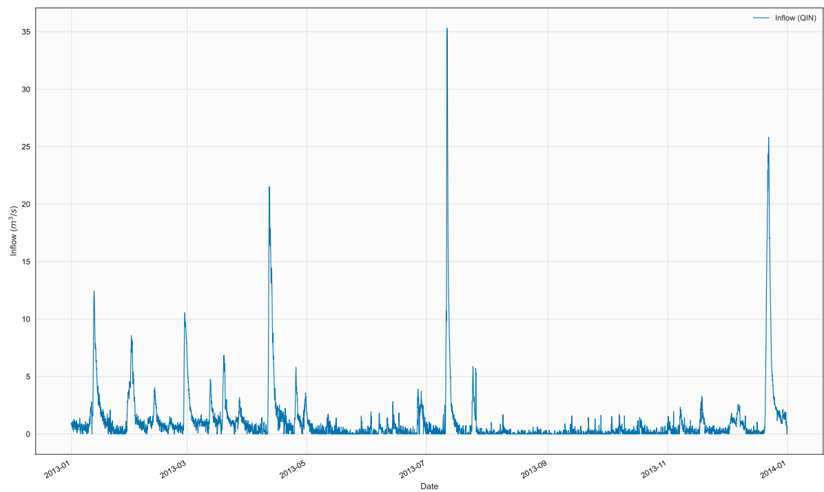
Figure 3. Time series of QIN, BR1, in file 2013_DeerCrk_Qin.npt
