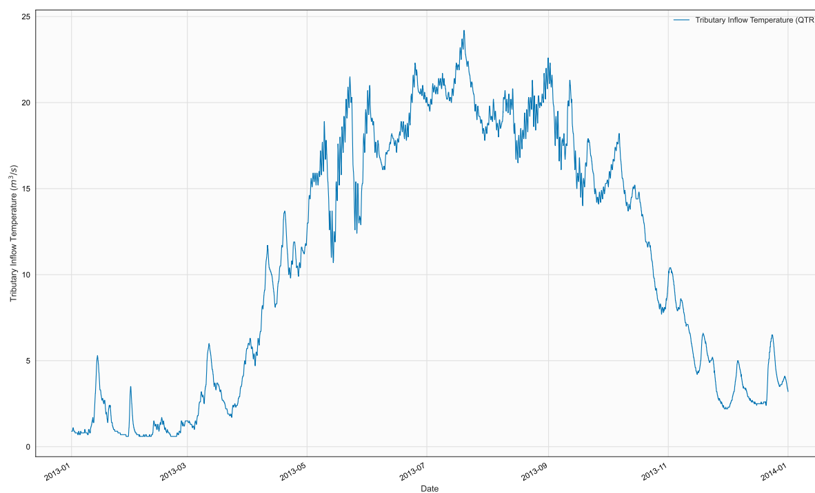
Figure 18. Time series of TTR, TR3, in file 2013_WBranch_Tin5.npt
