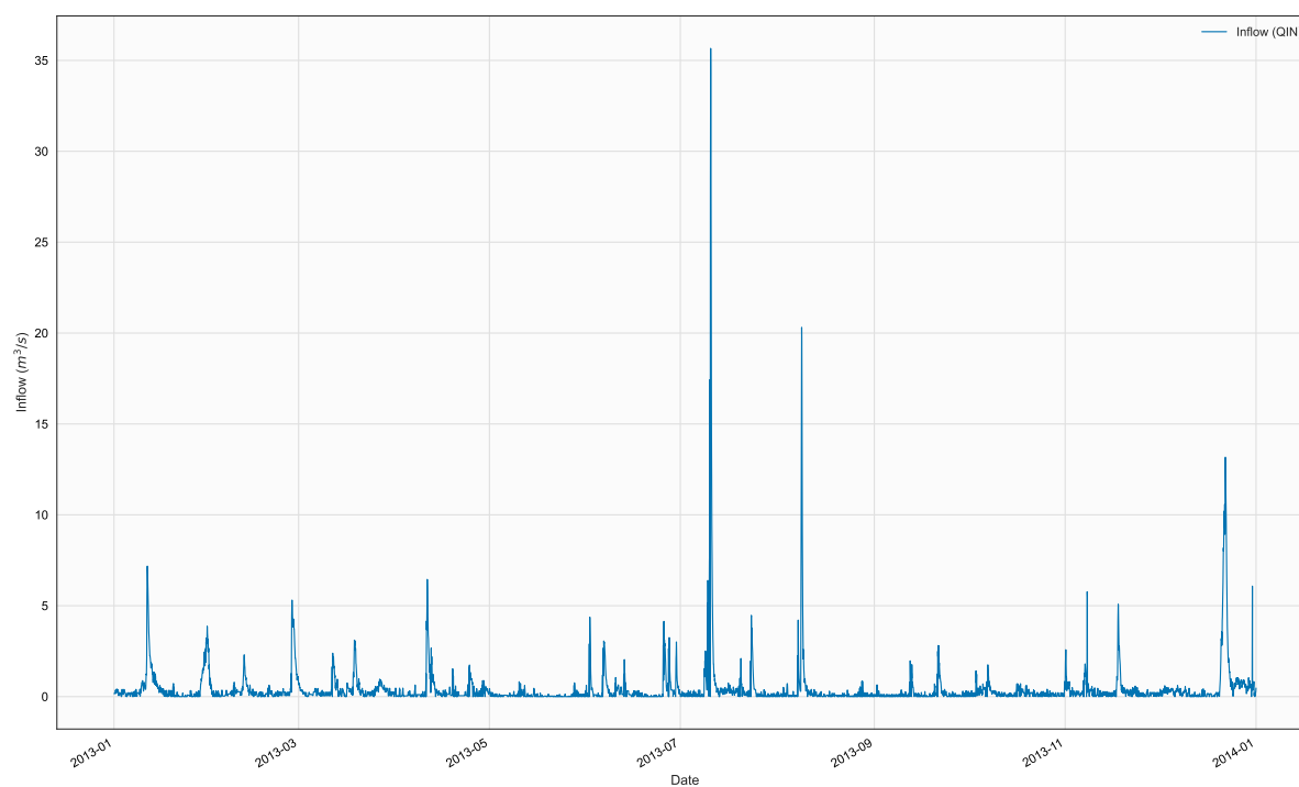
Figure 3. Time series of QIN, BR2, in file 2013_Silver_Qin.npt
