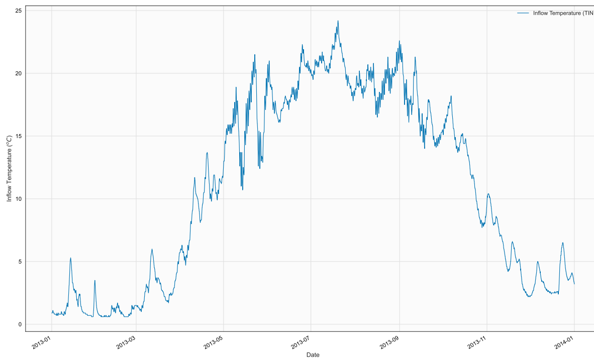
Figure 7. Time series of TIN, BR3, in file 2013_WBranch_Tin2.npt
