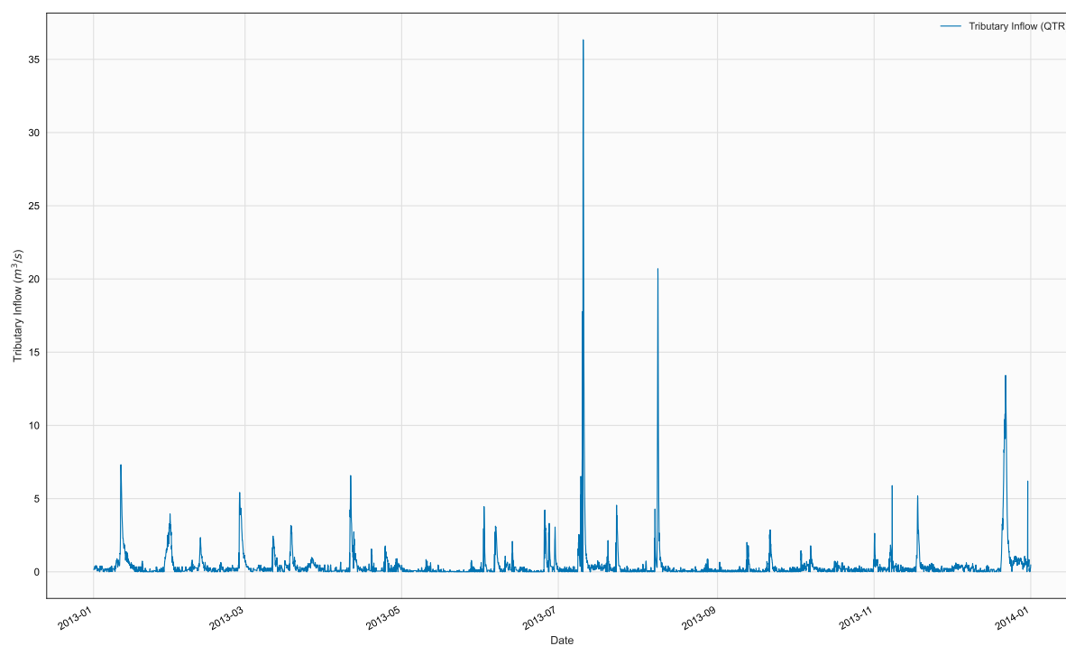
Figure 15. Time series of QTR, TR3, in file 2013_Hinkley_Qtr.npt
