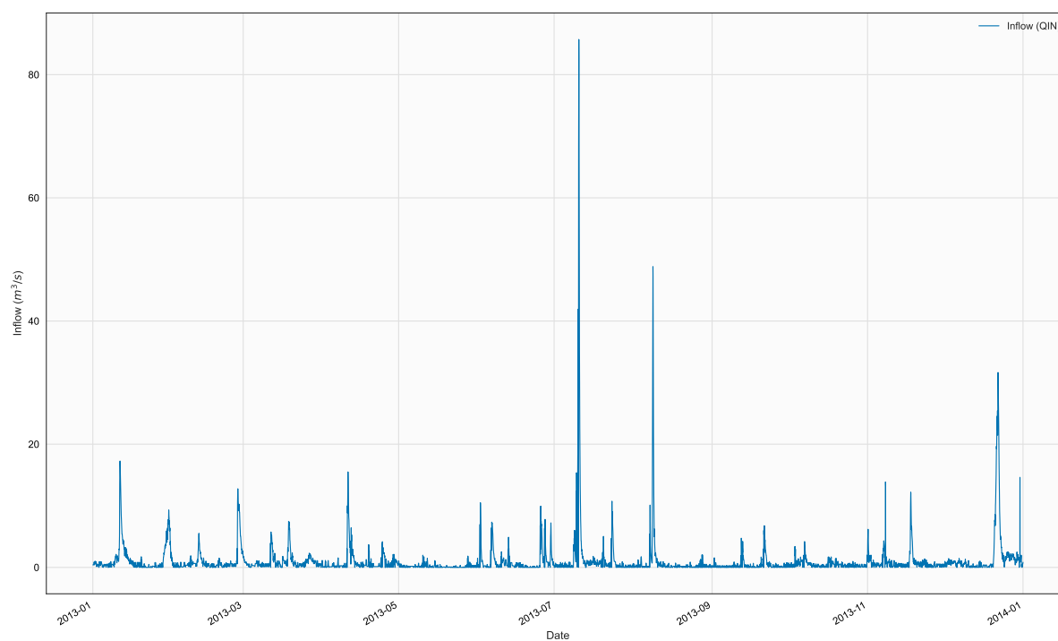
Figure 2. Time series of QIN, BR1, in file 2013_WBranch_Qin.npt
