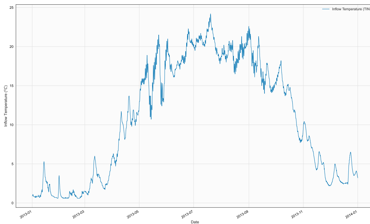
Figure 5. Time series of TIN, BR1, in file 2013_WBranch_Tin.npt
