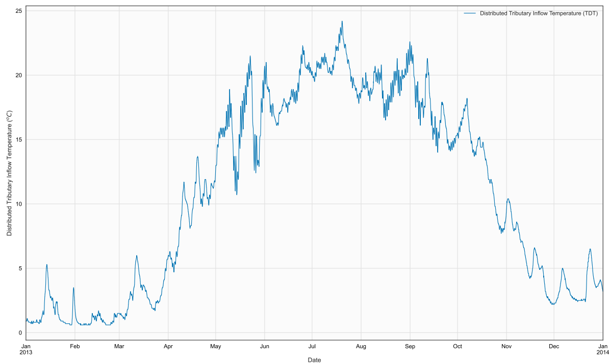
Figure 23. Time series of TDT, BR1, in file 2013_Ktdt.npt
