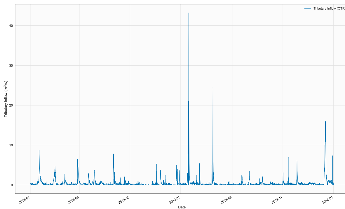
Figure 13. Time series of QTR, TR1, in file 2013_Barrel_Qtr.npt
