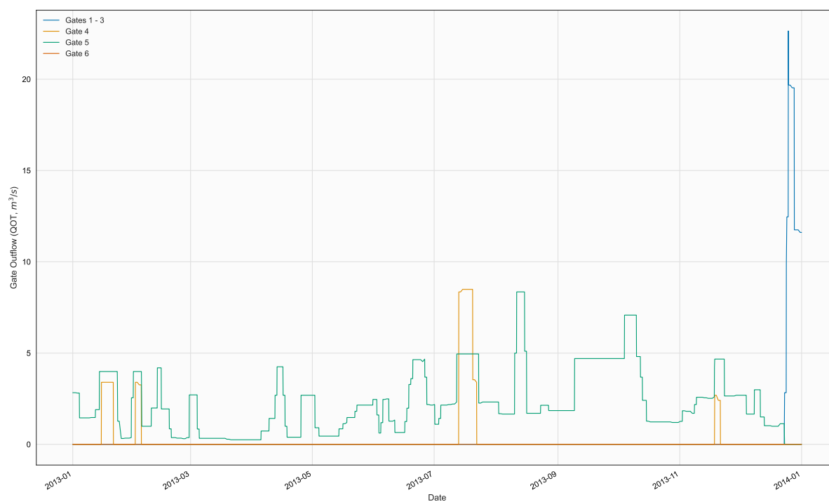
Figure 11. Time series of QOT, TR1, in file 2013_MJKirwanDam.npt
