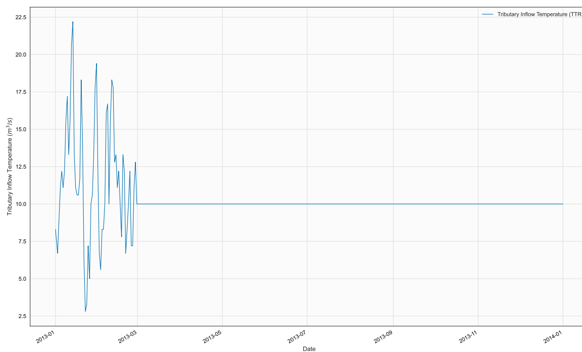
Figure 54. Time series of TTR, TR8, in file 2013_BDMWarren008_Ttr.npt
