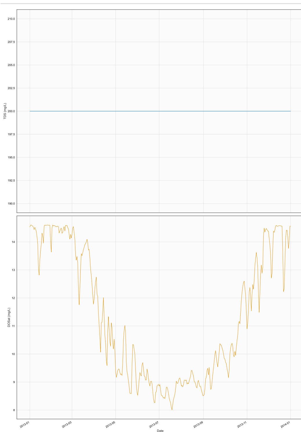
Figure 80. Time series of CTR, TR6, in file 2013_PtSource_Nodata2.npt
