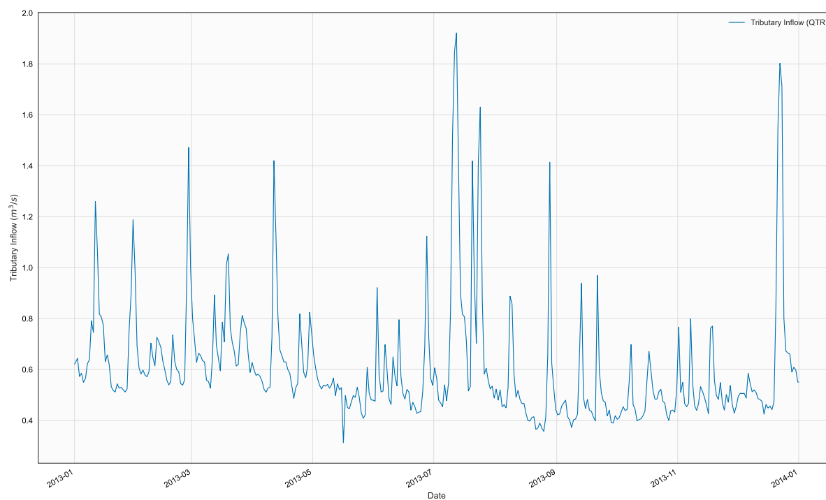
Figure 31. Time series of QTR, TR13, in file 2013_WarrenWpcf_Qtr.npt
