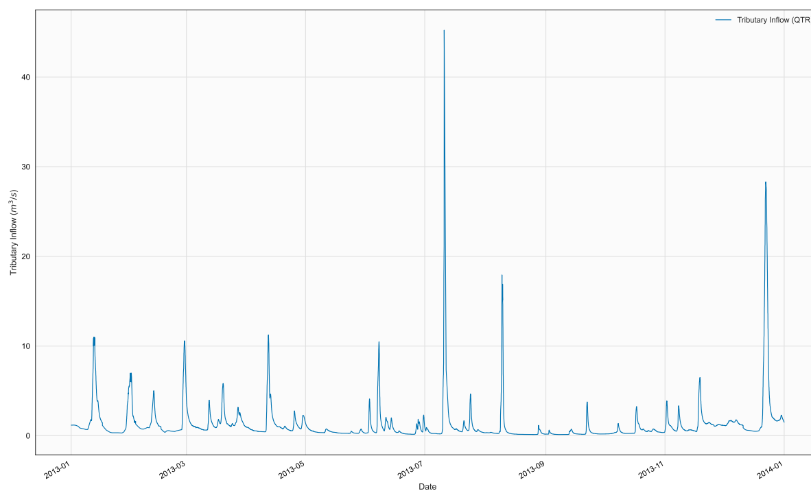
Figure 44. Time series of QTR, TR26, in file 2013_YellowCrk_Qtr_est15.npt
