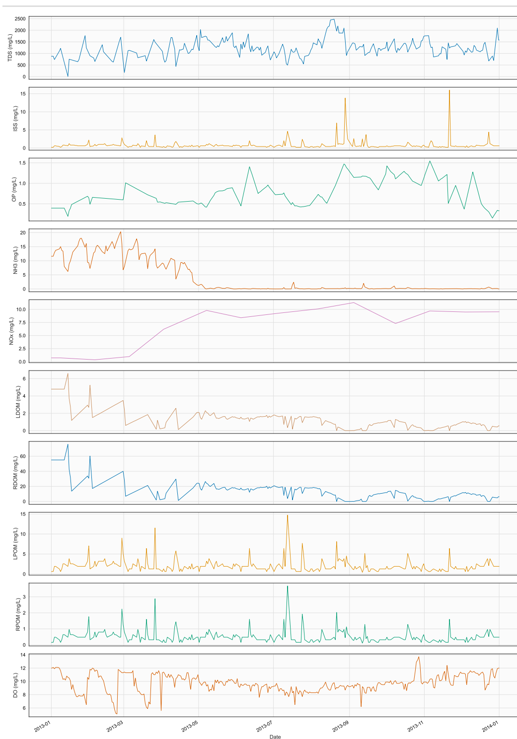
Figure 87. Time series of CTR, TR13, in file 2013_WarrenWpcf_Ctr.npt
