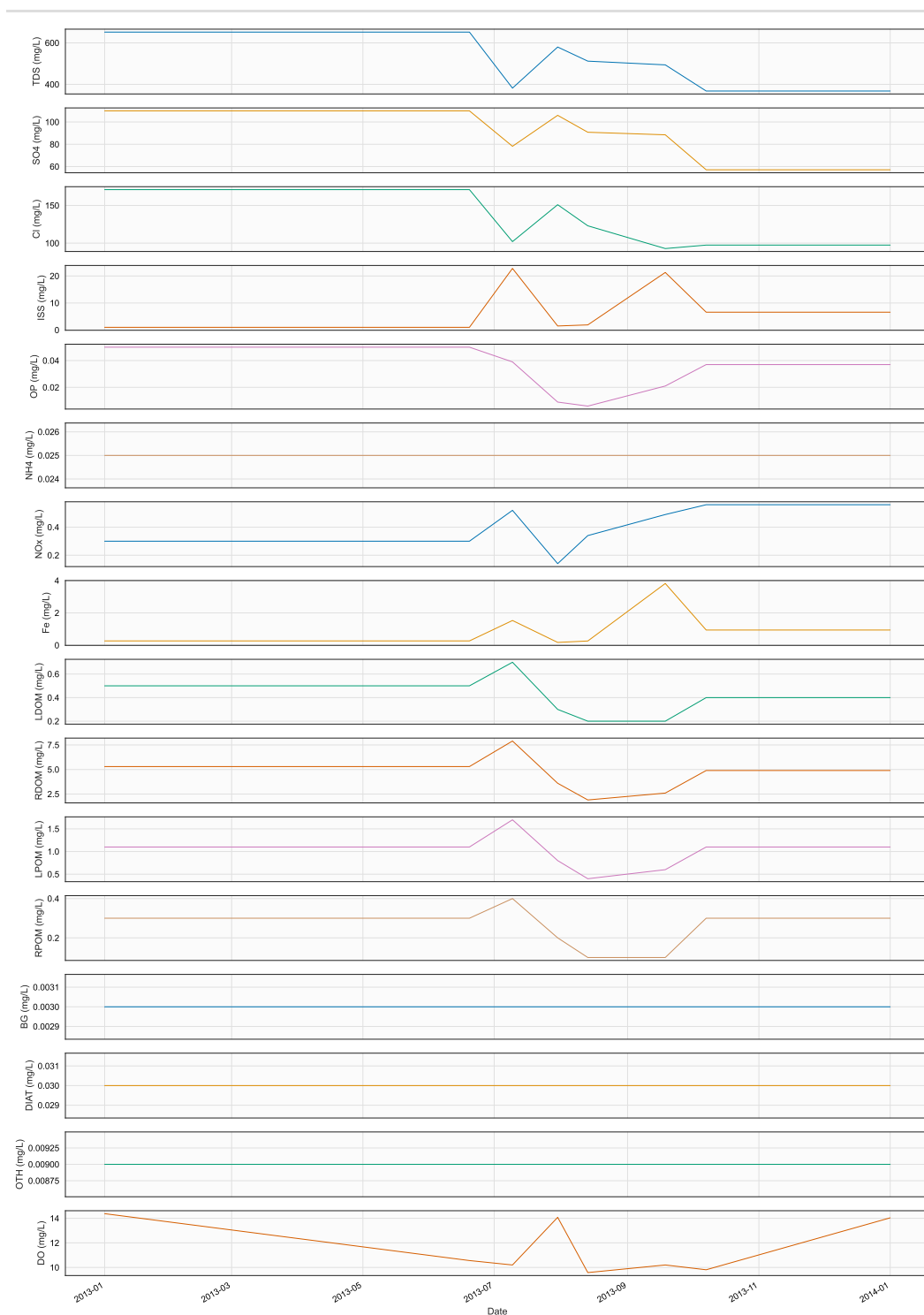
Figure 94. Time series of CTR, TR20, in file 2013_FourMile_Ctr.npt
