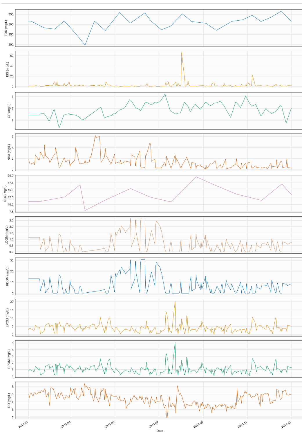
Figure 91. Time series of CTR, TR17, in file 2013_NilesWwtp_Ctr.npt
