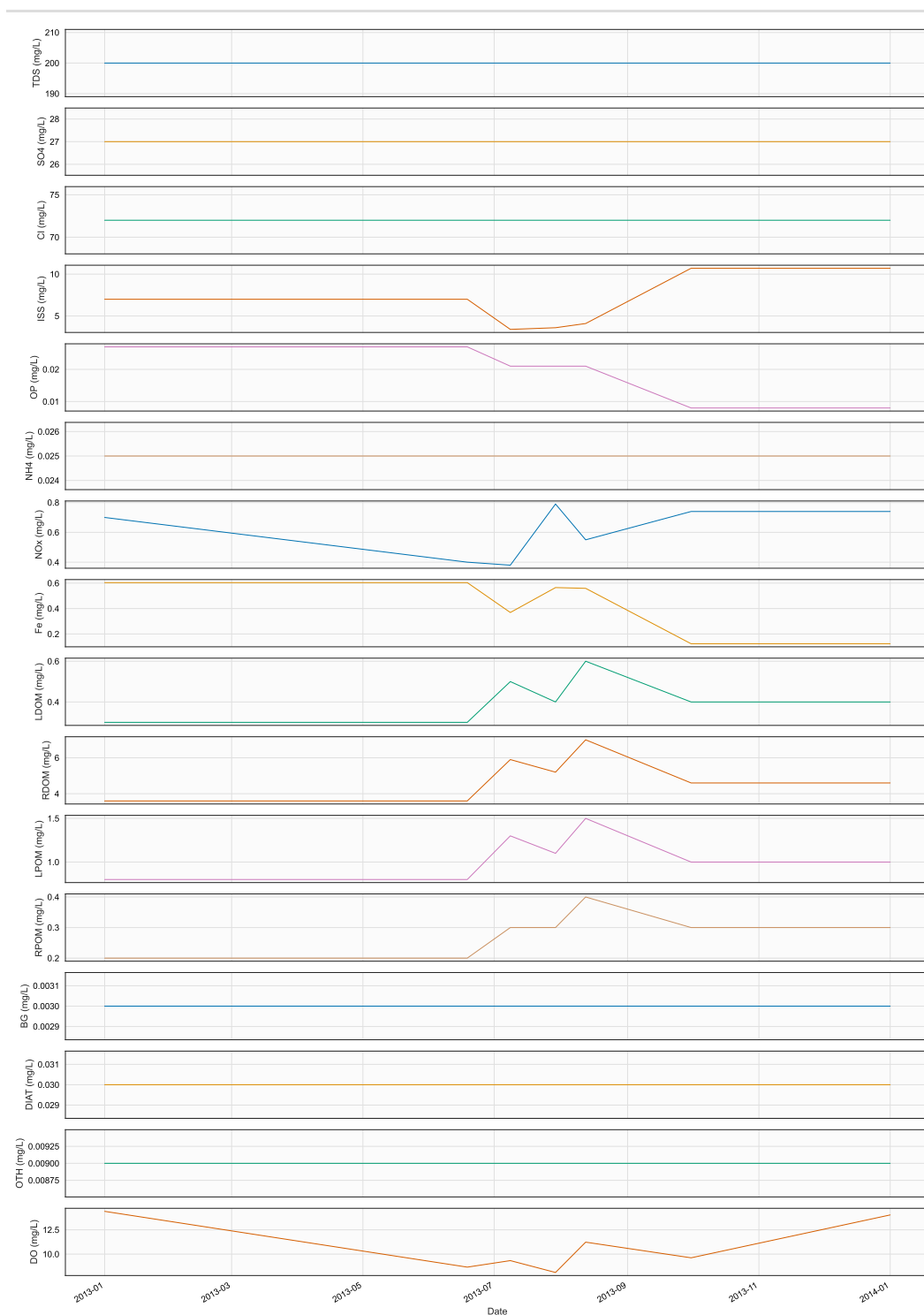
Figure 116. Time series of CDT, BR5, in file 2013_SquawCrk_Ctr2.npt
