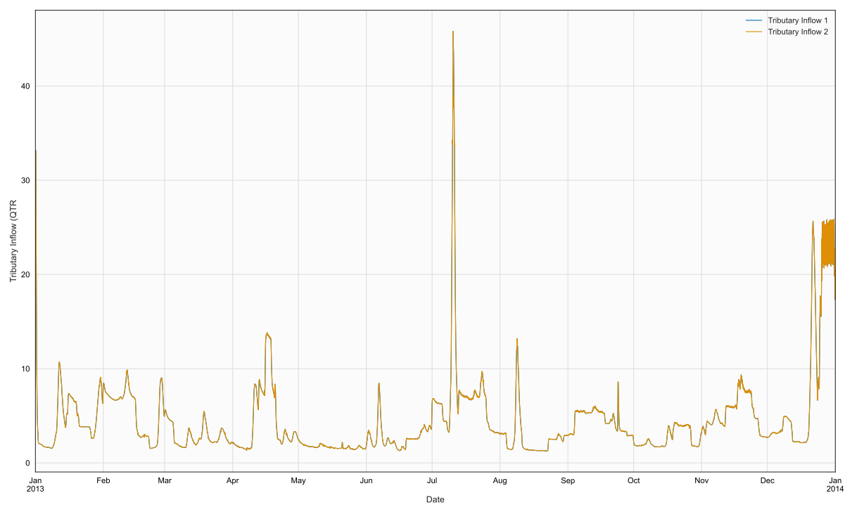
Figure 33. Time series of QTR, TR15, in file 2013_MosquitoCrkMouth_Qtr_est.npt
