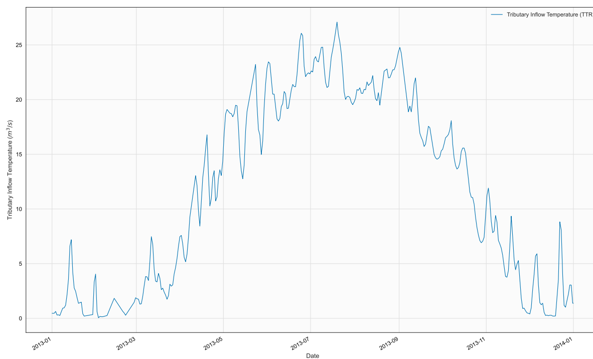
Figure 49. Time series of TTR, TR3, in file 2013_EagleCrk_Ttr_est.npt
