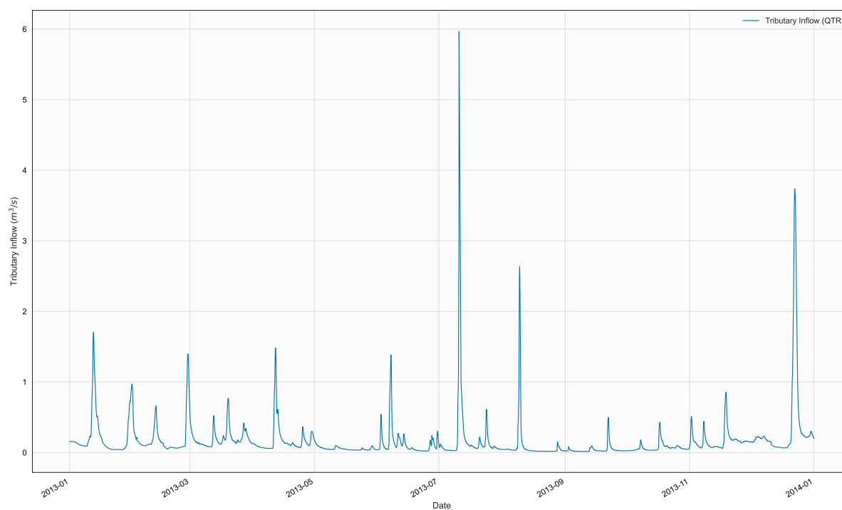
Figure 38. Time series of QTR, TR20, in file 2013_FourMileRun_Qtr_est15.npt
