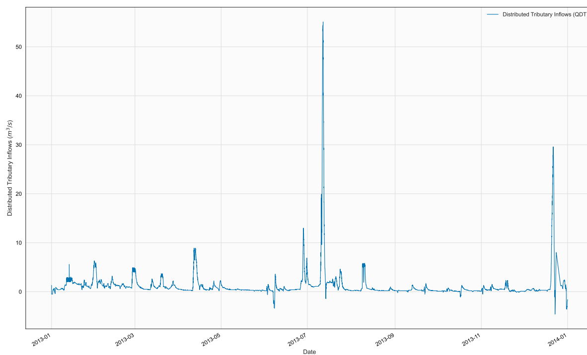
Figure 103. Time series of QDT, BR1, in file 2013_qdt_up1.npt
