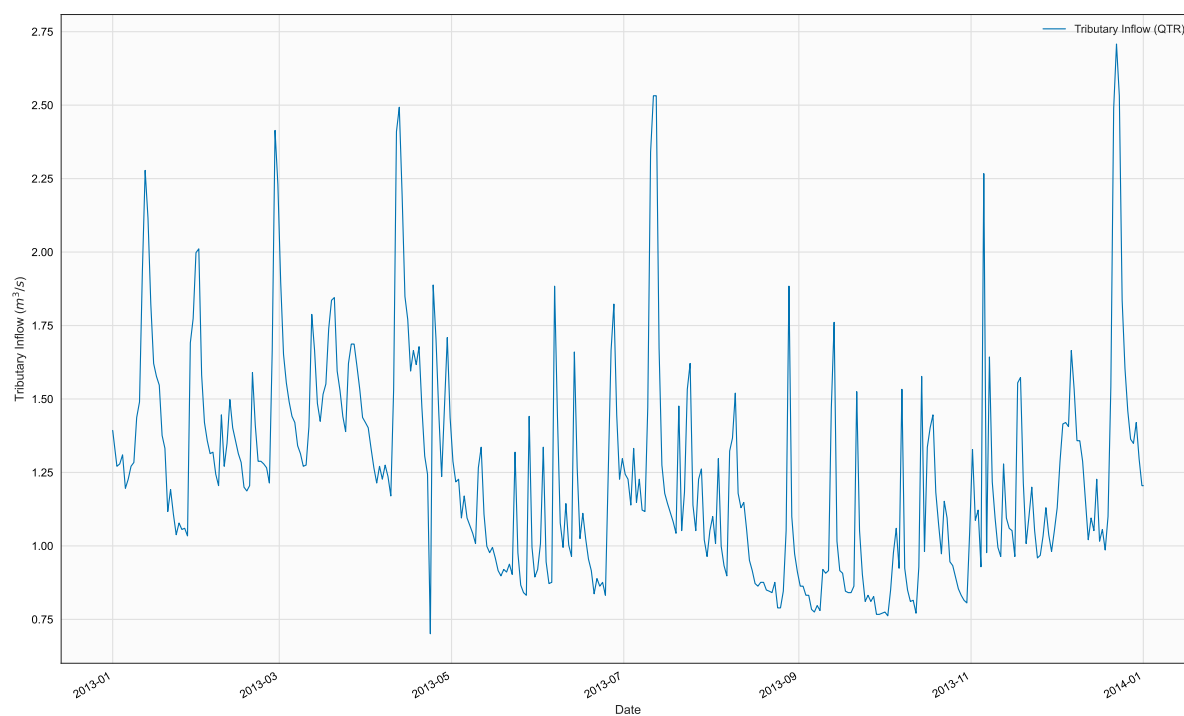
Figure 42. Time series of QTR, TR24, in file 2013_YoungstWwtp_Qtr.npt
