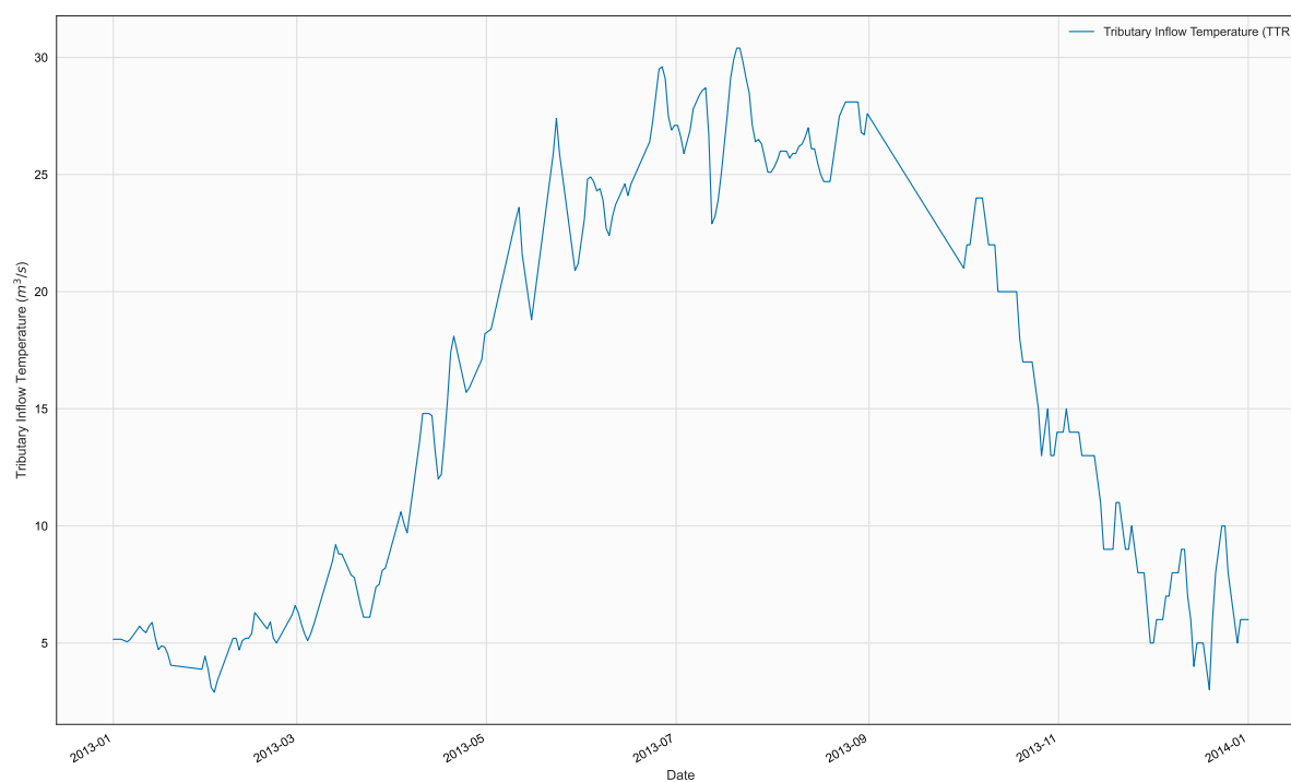
Figure 51. Time series of TTR, TR5, in file 2013_WarrenSteel005_Ttr.npt
