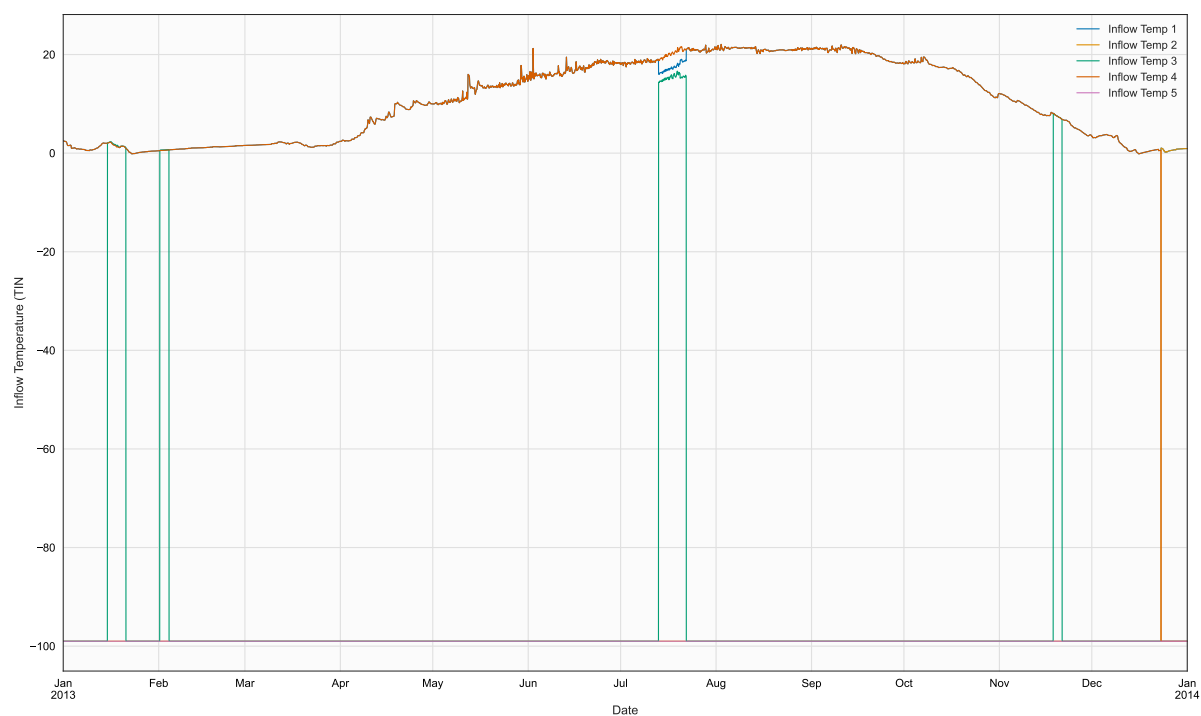
Figure 16. Time series of TIN, BR2, in file 2013_MJKirwan_Ttr.npt
