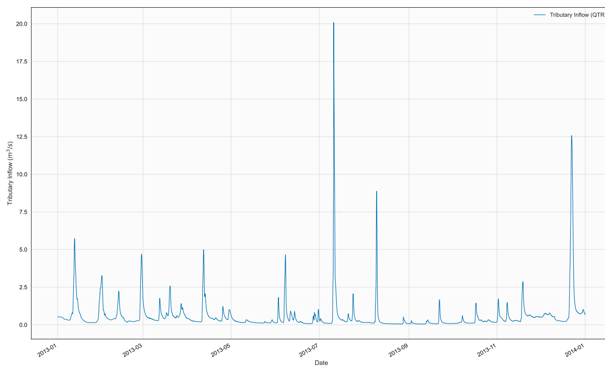
Figure 37. Time series of QTR, TR19, in file 2013_SquawCrk_Qtr_est15.npt
