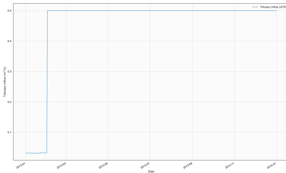
Figure 27. Time series of QTR, TR9, in file 2013_BDMWarren013_Qtr.npt
