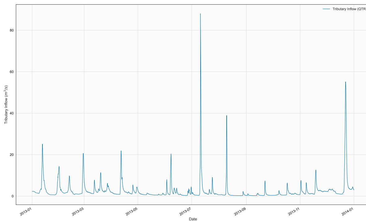
Figure 40. Time series of QTR, TR22, in file 2013_MillCrk_Qtr_est15.npt
