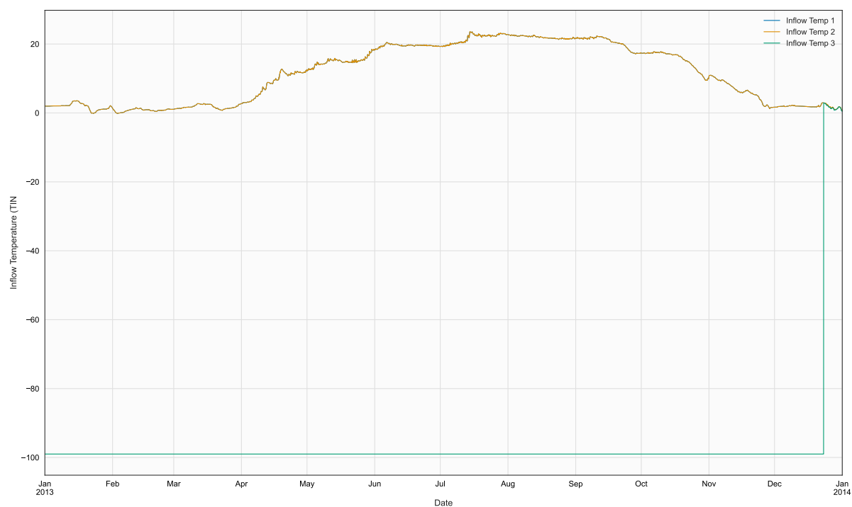
Figure 15. Time series of TIN, BR1, in file 2013_Milton_Tin.npt
