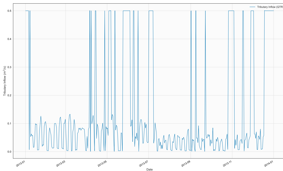
Figure 36. Time series of QTR, TR18, in file 2013_McDonald_Qtr.npt
