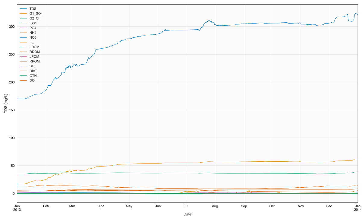
Figure 17. Time series of CIN, BR1, in file 2013_Milton_Cin.npt
