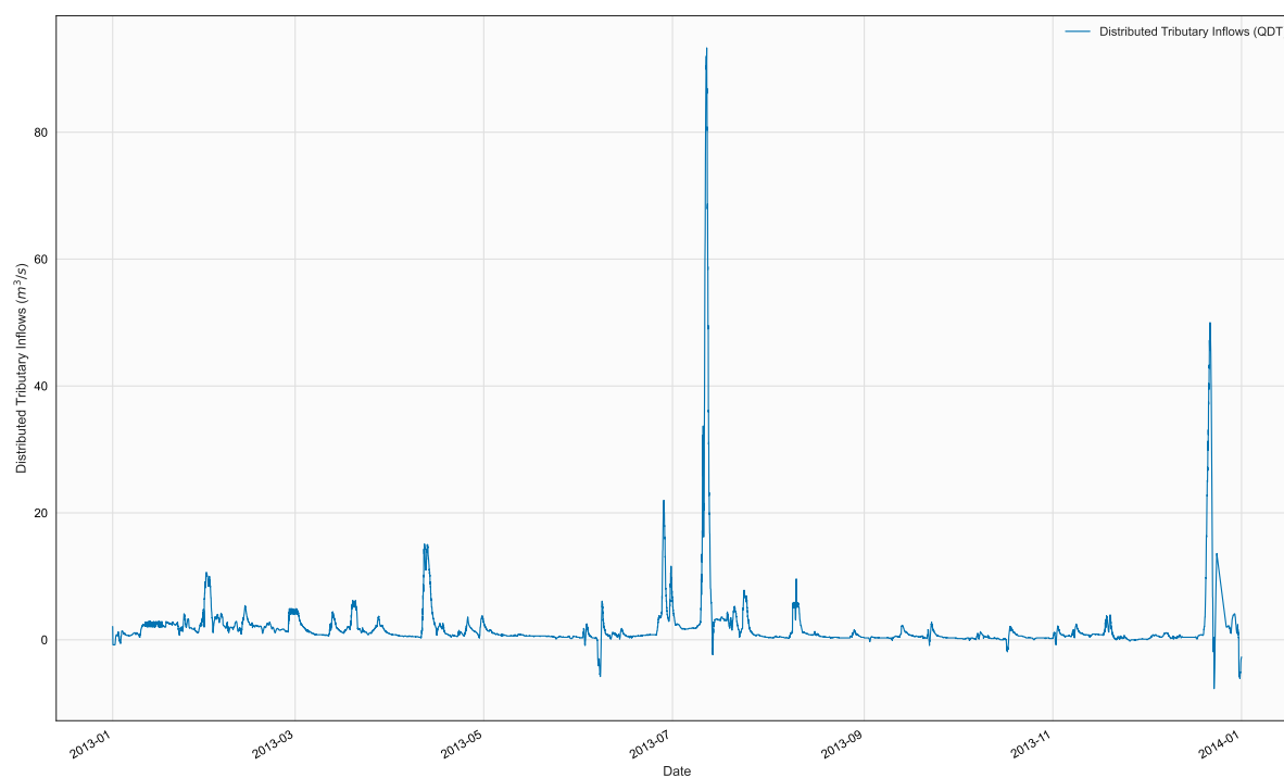
Figure 104. Time series of QDT, BR2, in file 2013_qdt_up2.npt
