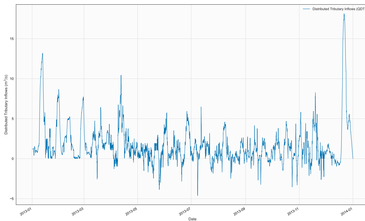
Figure 15. Time series of QDT, BR1, in file qwb_1_72hsm.npt
