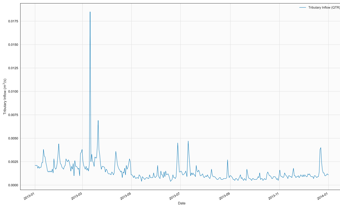
Figure 7. Time series of QTR, TR2, in file 2013_BazettaWwtp_Qtr.npt
