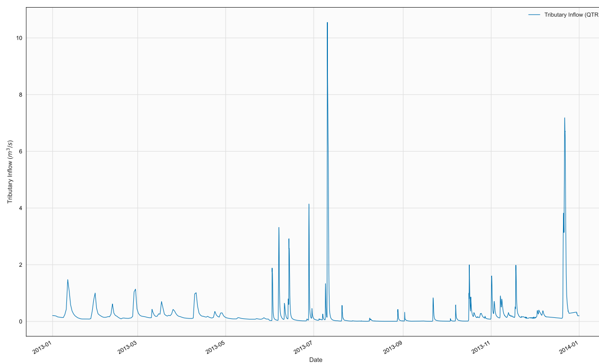
Figure 8. Time series of QTR, TR3, in file 2013_WalnutCrk_Qtr.npt
