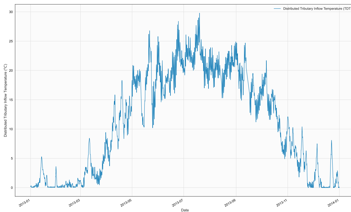
Figure 16. Time series of TDT, BR1, in file 2013_Tdt.npt
