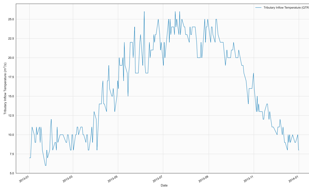
Figure 9. Time series of TTR, TR1, in file 2013_MeccaWwtp_Ttr.npt
