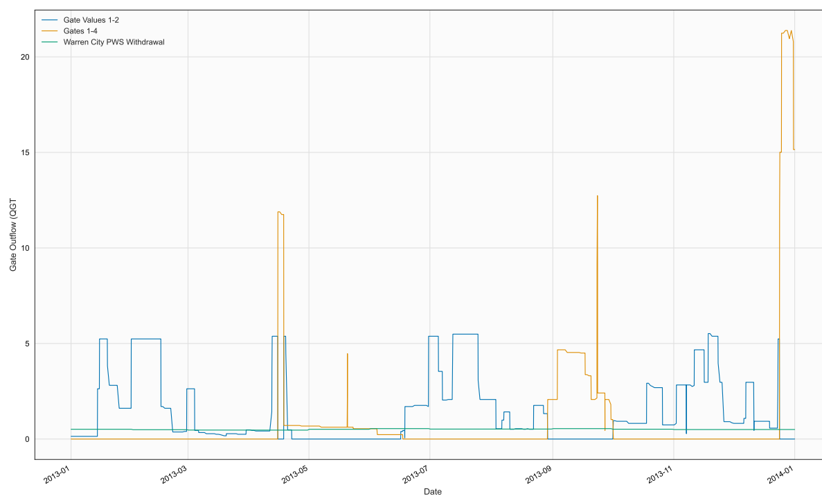
Figure 5. Time series of QGT, BR1, in file 2013_MosquitoDam.npt
