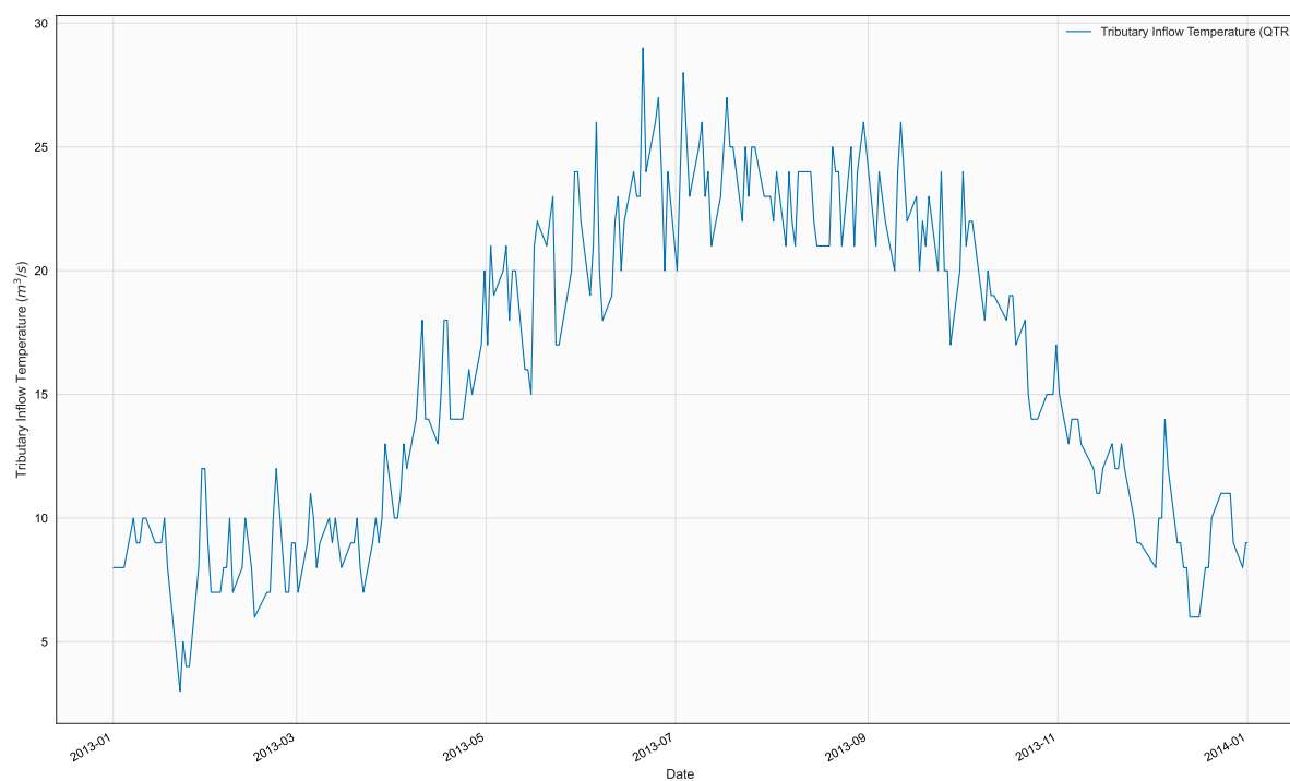
Figure 10. Time series of TTR, TR2, in file 2013_BazettaWwtp_Ttr.npt
