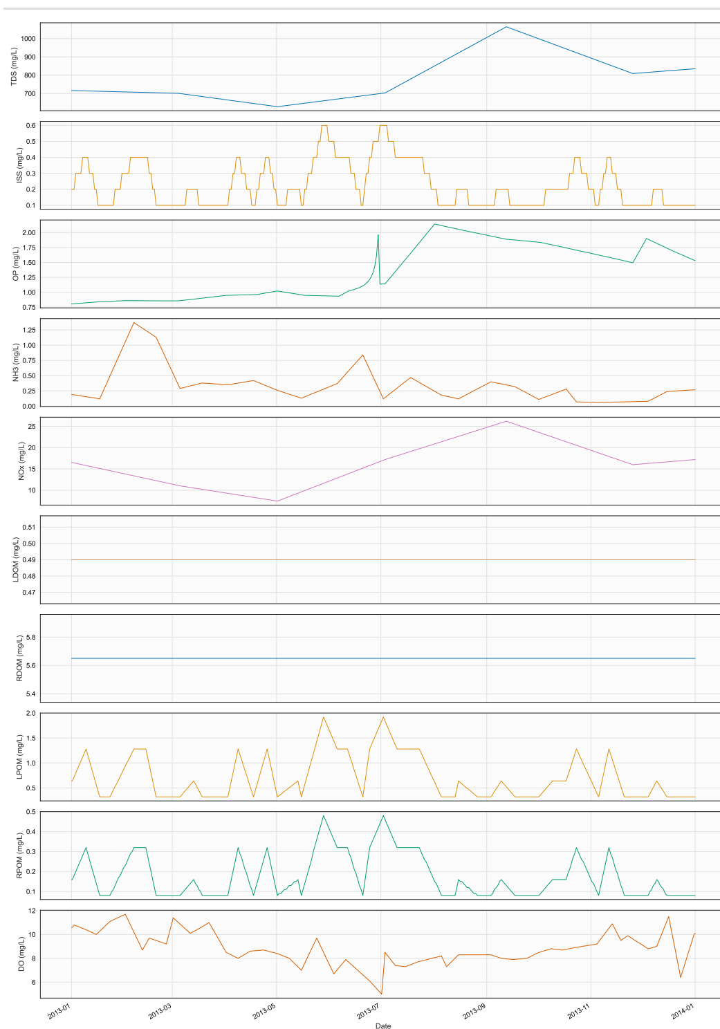
Figure 12. Time series of CTR, TR1, in file 2013_MeccaWwtp_Ctr.npt
