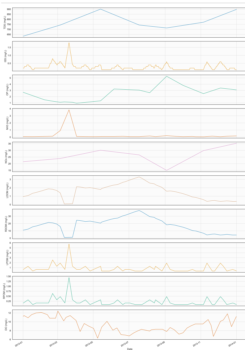
Figure 13. Time series of CTR, TR2, in file 2013_BazettaWwtp_Ctr.npt
