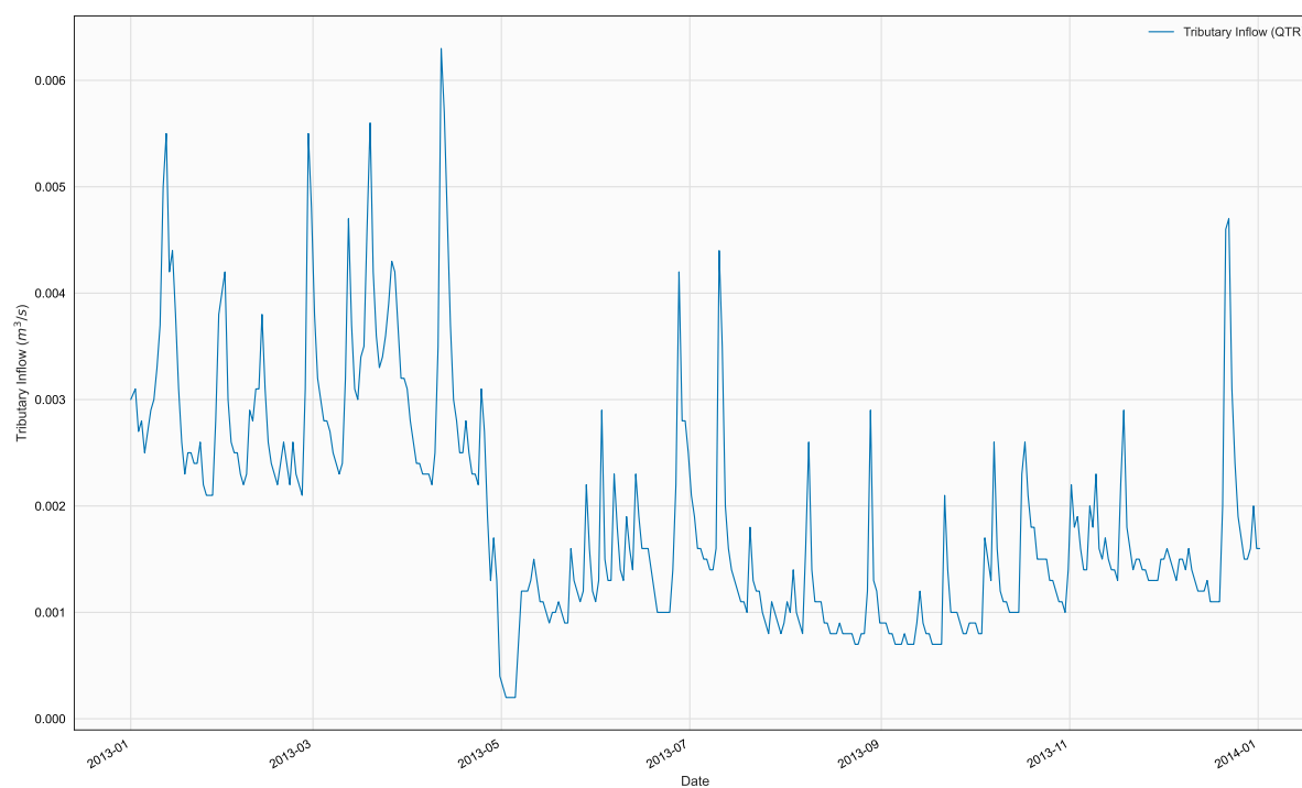
Figure 6. Time series of QTR, TR1, in file 2013_MeccaWwtp_Qtr.npt
