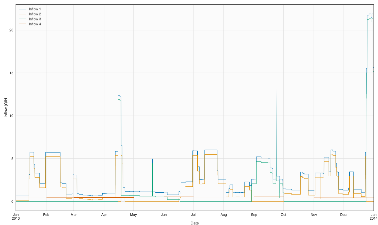
Figure 3. Time series of QIN, BR1, in file 2013_MosquitoDam_Qwo.npt
