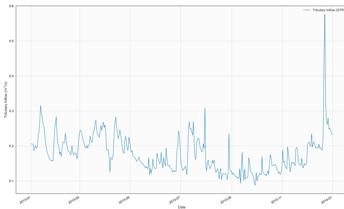
Figure 6. Time series of QTR, TR1, in file 2013_TrumbullWwtp_Qtr.npt
