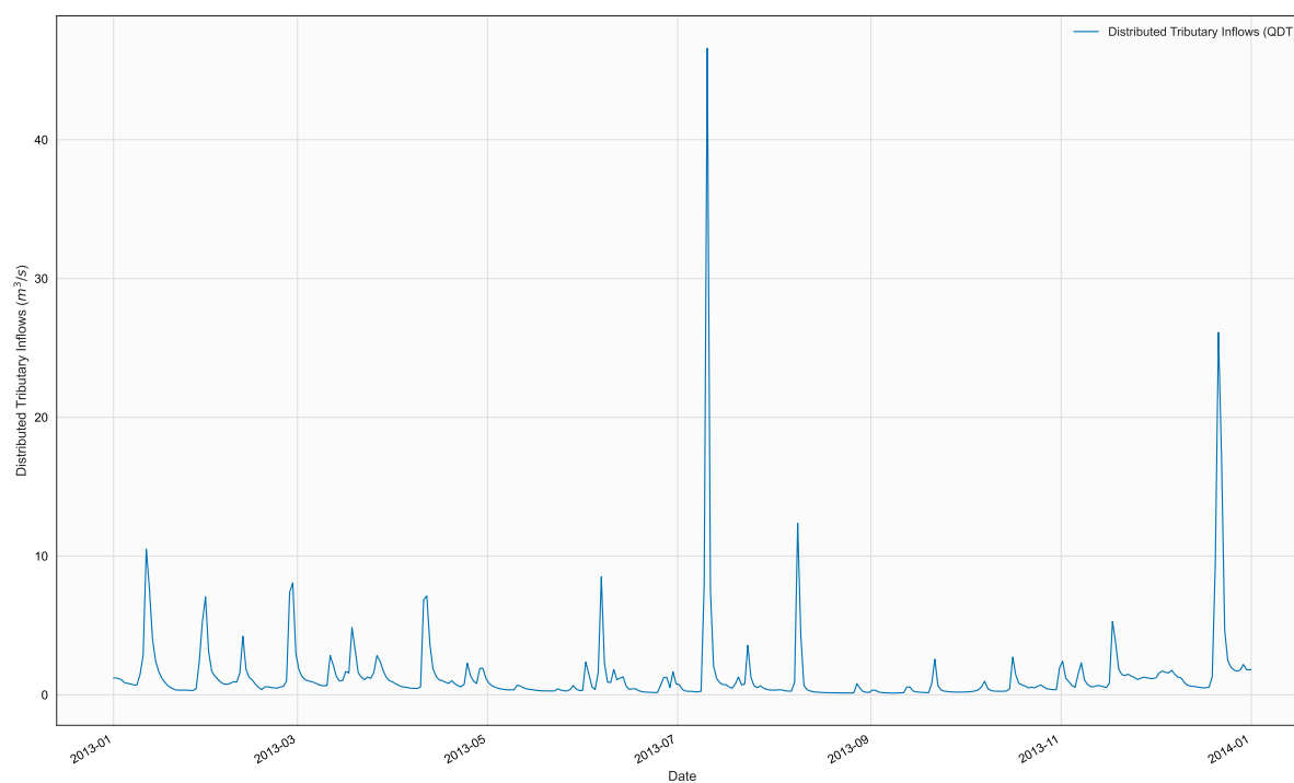
Figure 9. Time series of QDT, BR1, in file 2013_Qdt.npt
