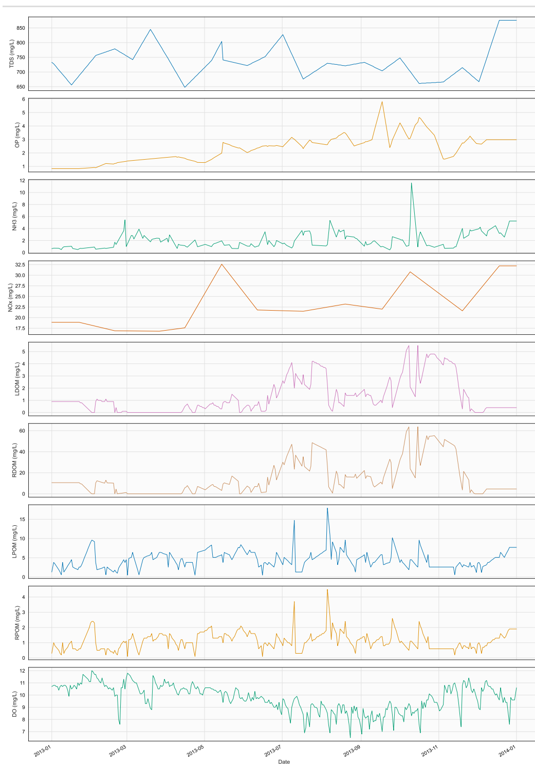
Figure 8. Time series of CTR, TR1, in file 2013_TrumbullWwtp_Ctr.npt
