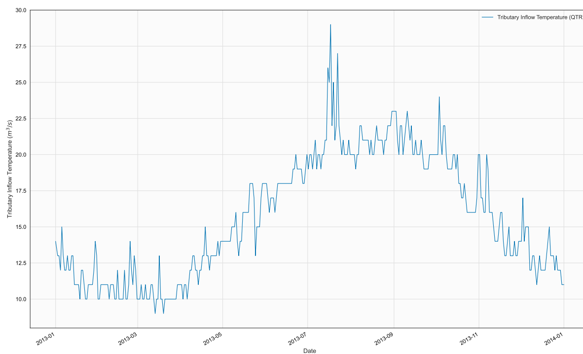
Figure 7. Time series of TTR, TR1, in file 2013_TrumbullWwtp_Ttr.npt
