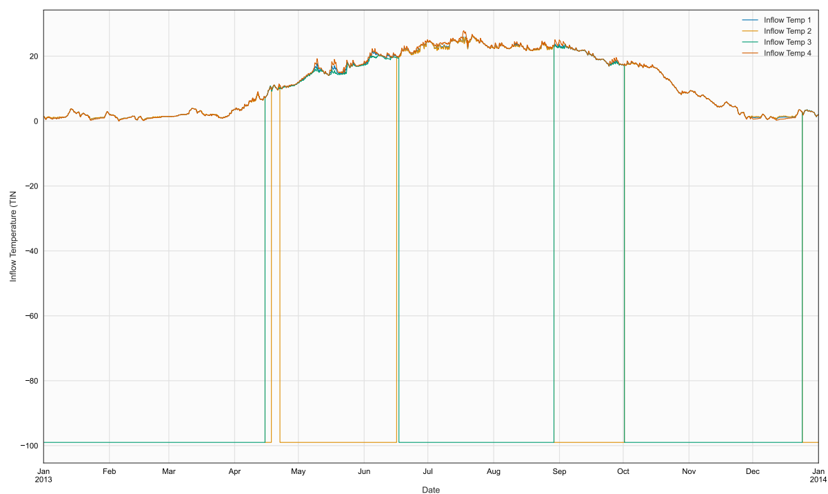
Figure 4. Time series of TIN, BR1, in file 2013_MosquitoDam_Two.npt
