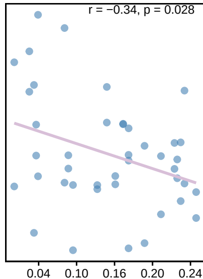
Pollinators overlap
