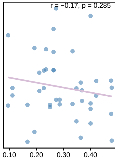
Plants overlap
