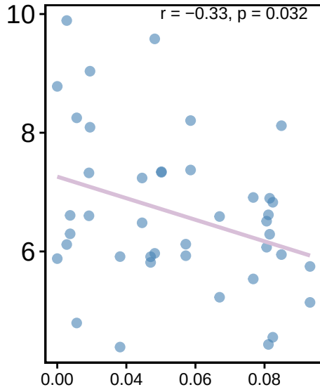
Interaction overlap
