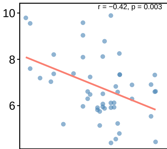
Network size
