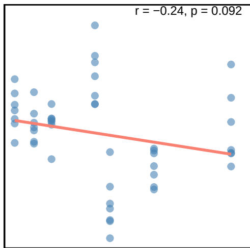
Density of matrix P
