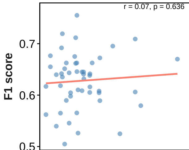
Density of matrix C
