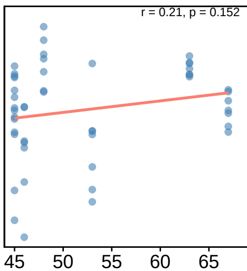
Network size
