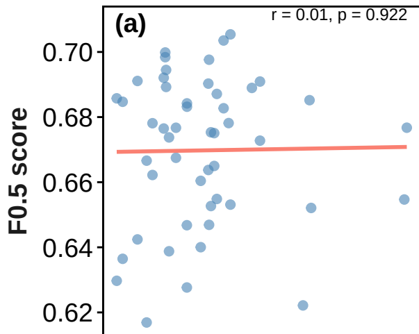
Connectance of matrix C
