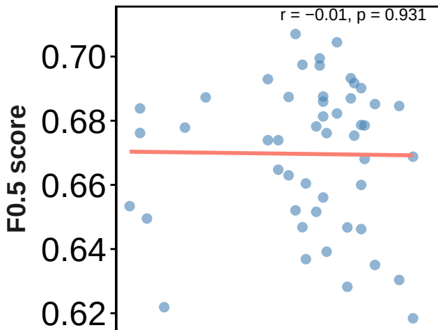
Size of matrix C
