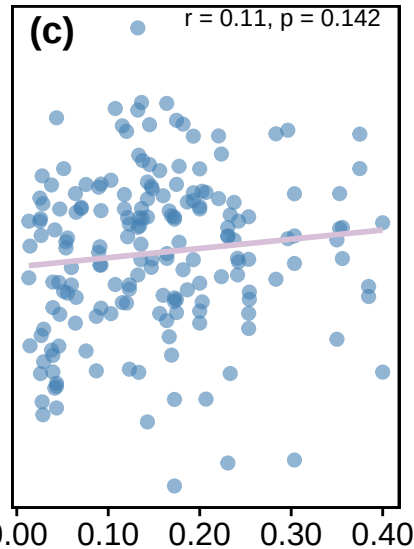
Pollinators overlap
