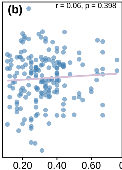
Plants overlap
