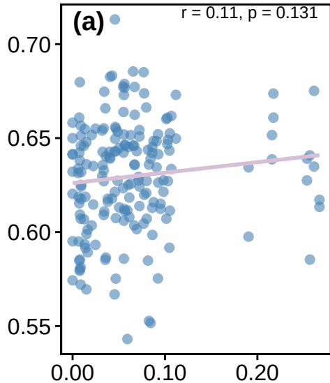
Interaction overlap
