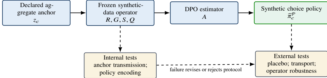
Figure 1: The paper’s scientific object. Solid arrows construct a policy. Dashed arrows are tests, not guarantees. A failed test rejects a claim about this protocol; it does not prove that a population lacks the relevant preference.
