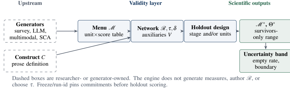
Figure 2: Epistemic systems view. Generators expand the menu; the validity layer adjudicates it; scientific conclusions are the image of a target functional on survivors, with additive sampling diagnostics.
