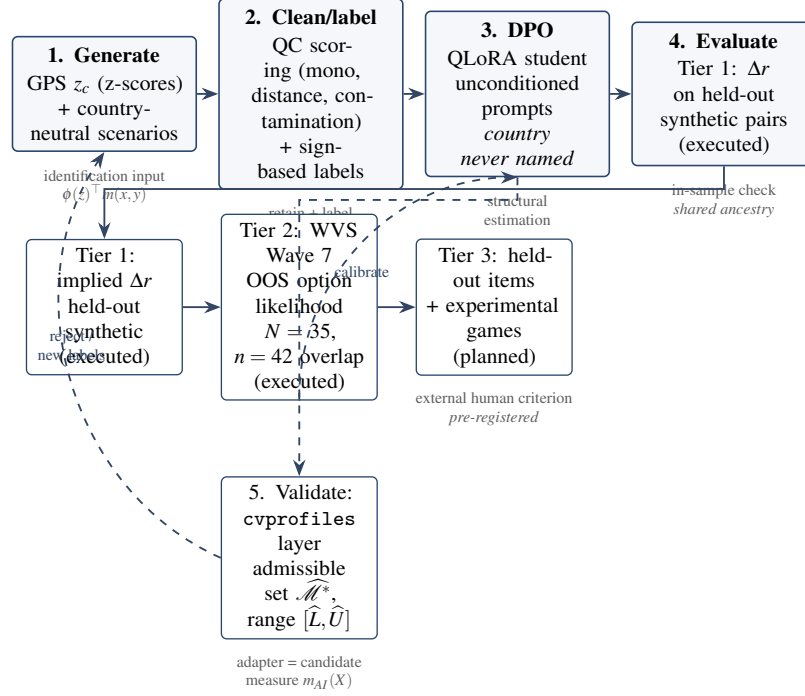
Figure 1: SCA 2.0 as a latent-structural-modeling system. Solid arrows are executed; dashed arrows are the planned validation feedback loops. The GPS state enters only as training labels (“the country is never named”), so cultural dispositions are encoded into weights, not prompts. Evaluation proceeds through three pre-registered tiers: synthetic recovery (Tier 1), out-of-sample WVS option likelihood against an external human criterion (Tier 2), and held-out items plus experimental games (Tier 3, planned). The cvprofiles layer admits the adapter itself as a candidate measurement function m_{AI}(X) and returns the admissible set \hat{\mathcal{M}}^* and construct-identified range [\hat{L}, \hat{U}] .
