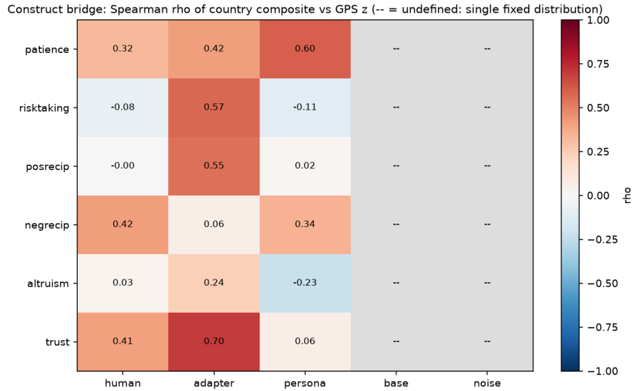
Figure 3: Construct bridge: Spearman \rho of the country composite versus the GPS country z-score, by dimension and model family. Gray cells are undefined (base and noise are single fixed distributions with no cross-country composite variation). The trust row is the paper’s positive result: adapter 0.70, human layer 0.41, persona prompt 0.06. Human layer n = 42 ; adapter and persona layers n = 16 .
