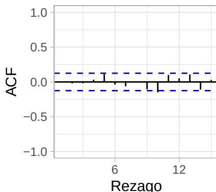
FAC residuos ARMA(1
