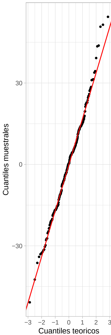
Q-Q plot residuos ARI
