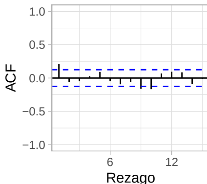
FAC residuos ARMA(2
