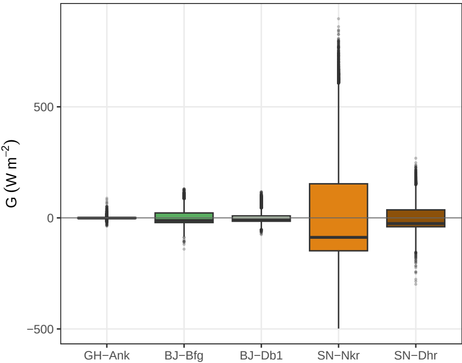
(c) Distribution of G by site, full record (BJ–Nhu excluded)
