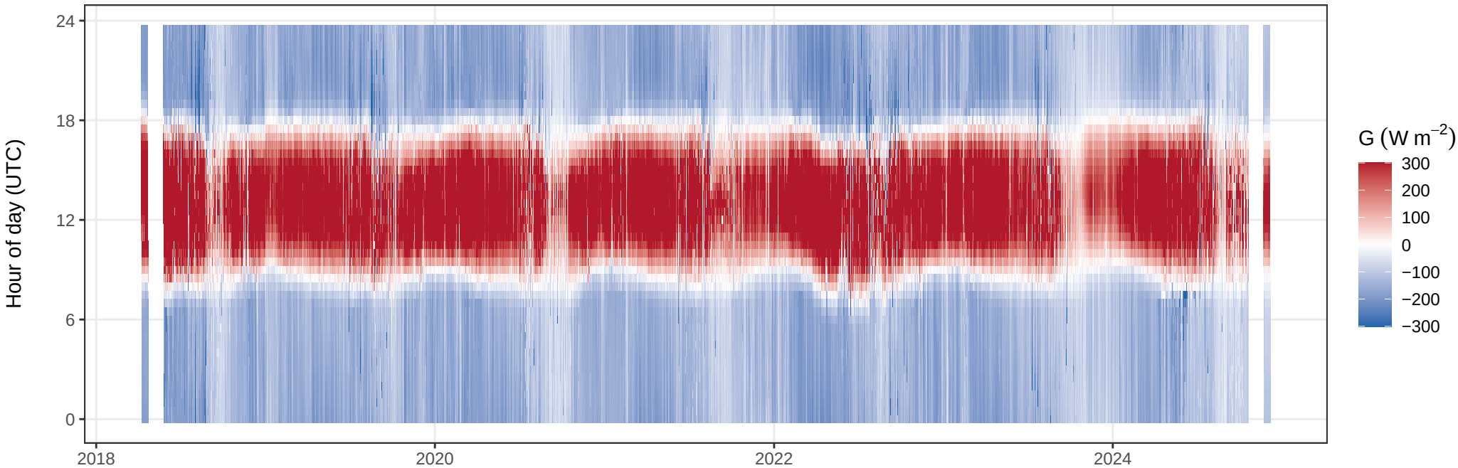
(d) SN–Nkr: G by date and hour of day (color capped at \pm 300 \text{ W m}^{-2} ; values to \pm 860 \text{ W m}^{-2} occur)
