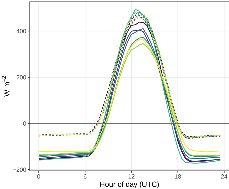
(a) SN–Nkr: mean diurnal composite of G and Rn, by year
