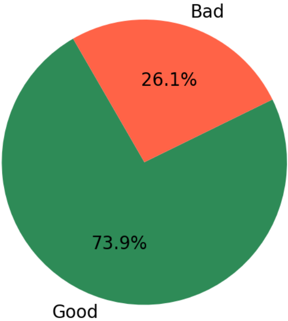
Feedback Distribution
