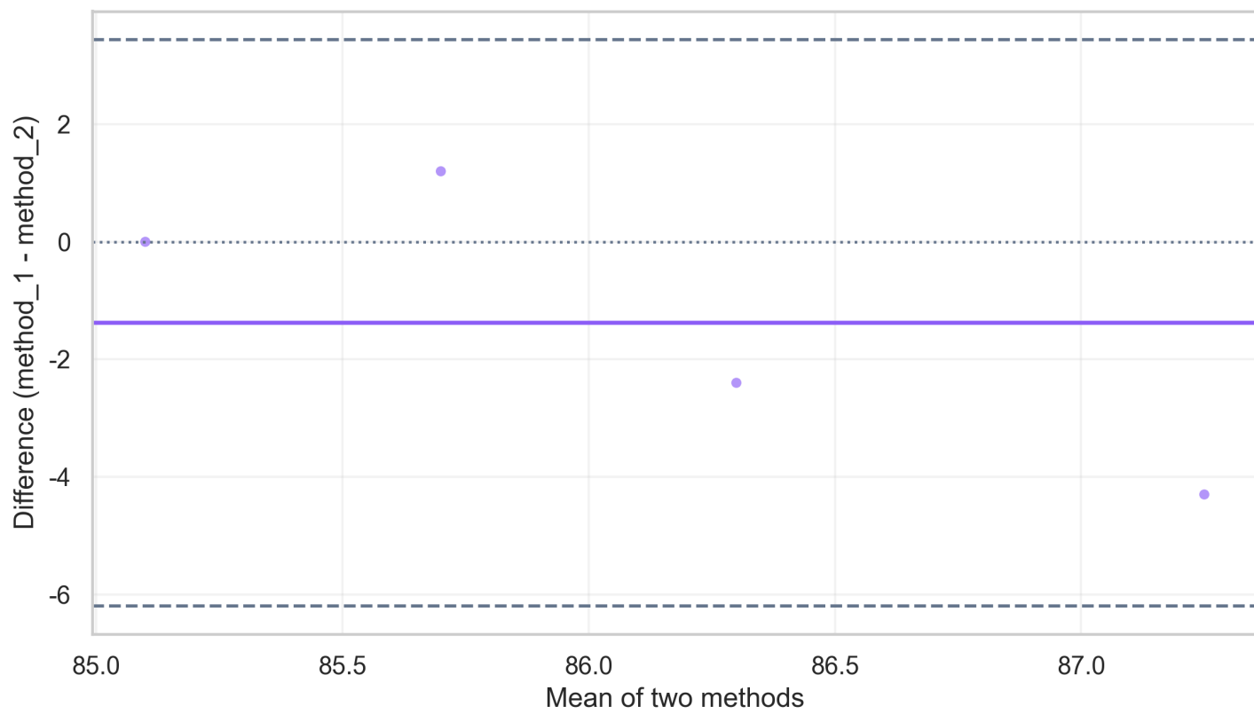
Bland-Altman Plot
