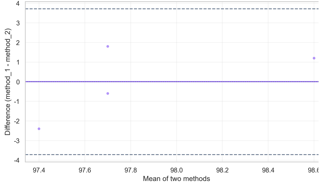
Bland-Altman Plot
