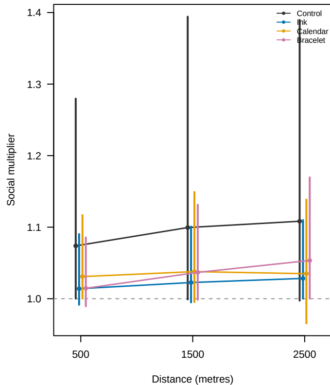
F3 two-stage conditional
