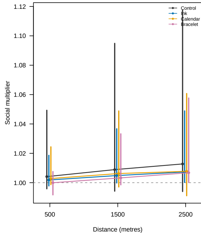
U3 two-stage unconditional
