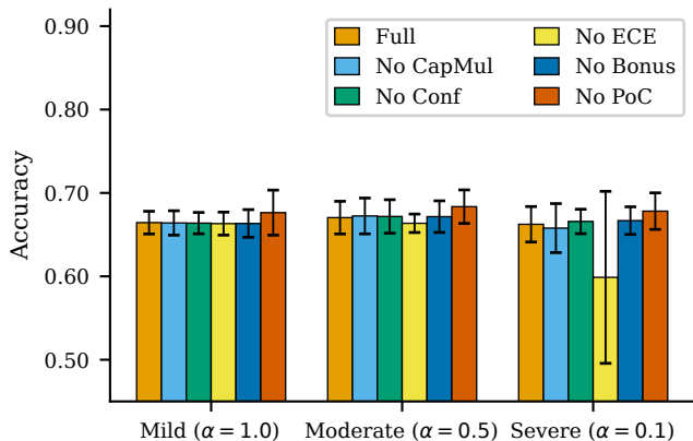
Ablation study — accuracy per component removed — DermaMNIST (mean \pm std, 5 seeds)
