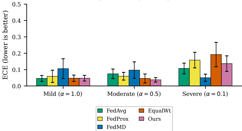
Calibration error by method and non-IID level — DermaMNIST (mean \pm std, 5 seeds)
